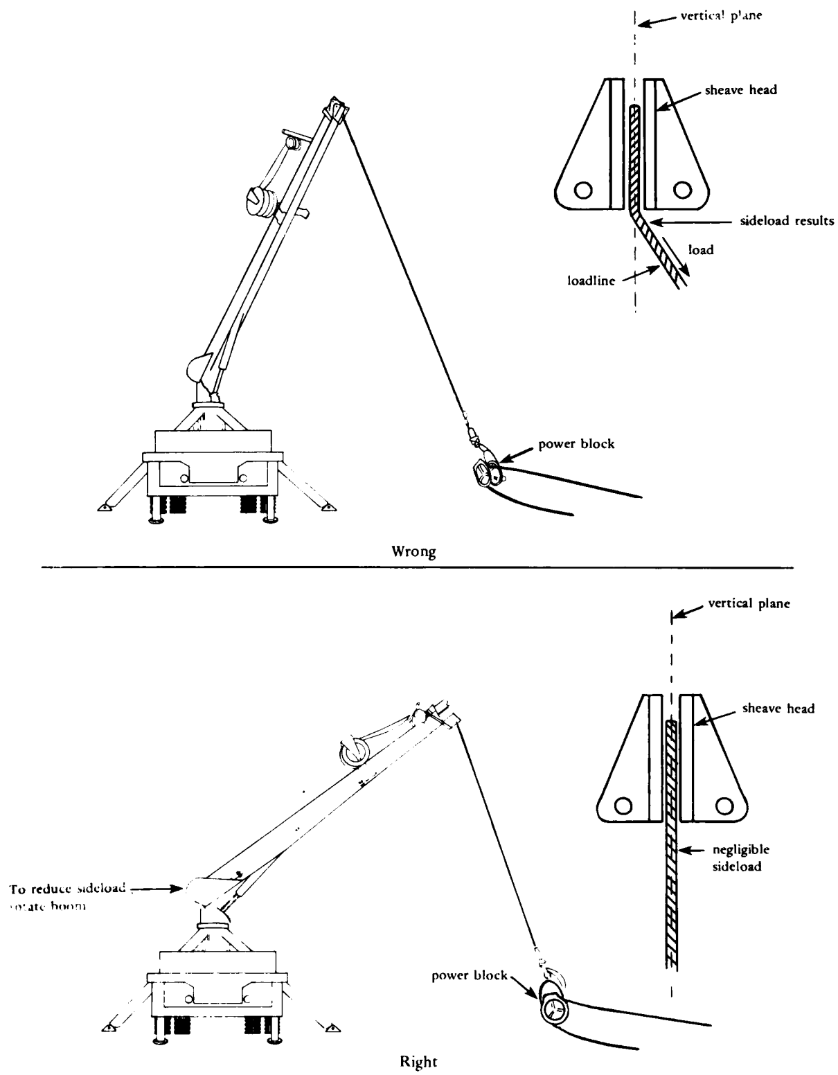
Figure 7-5. Minimizing boom sideloads.
