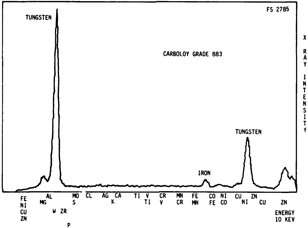
Figure 13. Typical Kevex Spectrograph - Carboloy Grade 883 Carbide.
