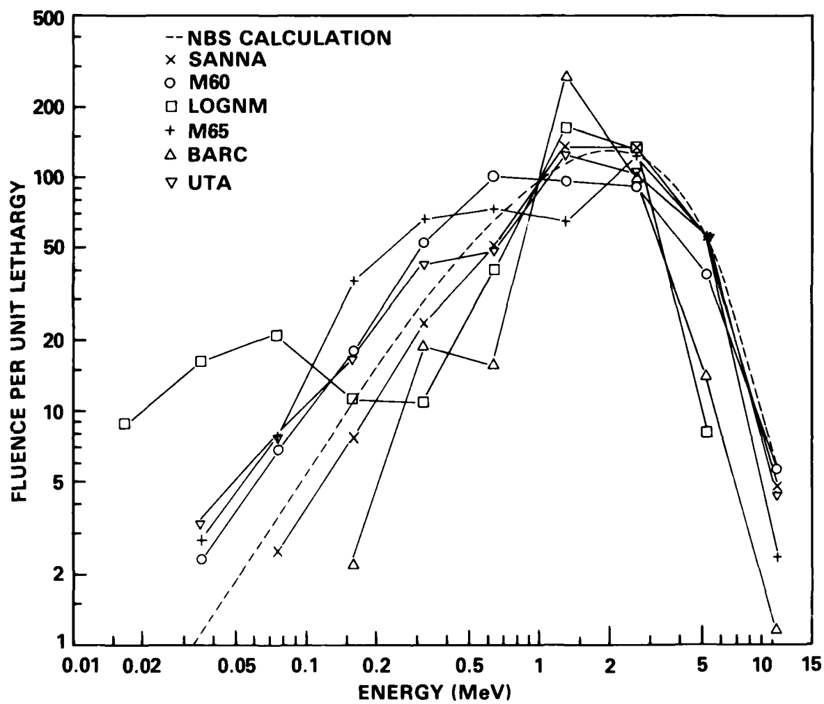
Fig. 1 Cf-252 neutron spectra obtained using each of the the response matrices in the YOGI unfolding code. The spectra were unfolded using the NBS calculation as the starting spectrum for YOGI.
