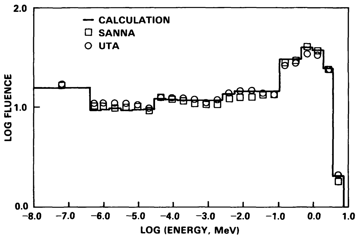
Fig. 2a Cf-252 room-return spectrum obtained using the SAN4 and UTA4 response matrices. The calculated spectrum was used as the starting spectrum for YOGI and the unfolded spectra were smoothed to the calculated spectrum.
