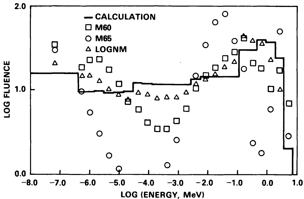
Fig. 2b Cf-252 room-return spectra obtained using the M60, M65, and LOGNM response matrices. The calculated spectrum was used as the starting spectrum for YOGI and the unfolded spectra were smoothed to the calculated spectrum.
