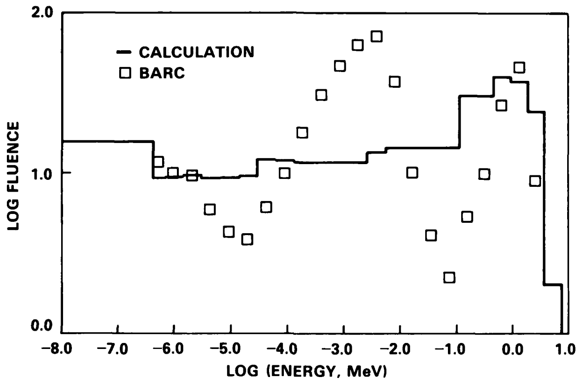
Fig. 2c Cf-252 room-return spectra obtained using the BARC response matrix. The calculated spectrum was used as the starting spectrum for YOGI and the unfolded spectrum was smoothed to the calculated spectrum.
