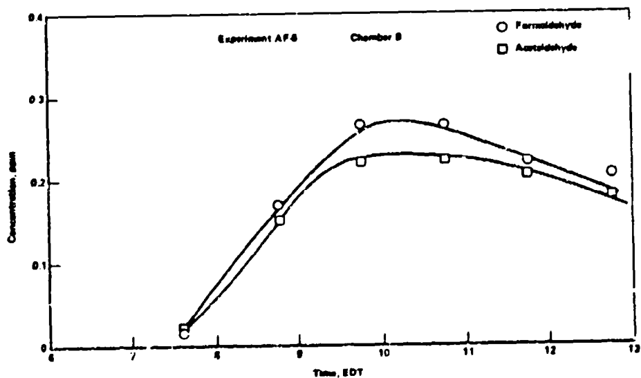
Figure A-12. Smog Chamber Profiles from AF-5 Using TF-39 Engine and JP-8 Shale-Derived Fuel (Reference Chamber)
