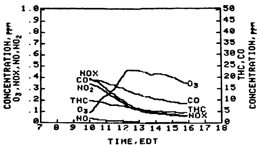
Figure A-20. Profiles from AF-9 Reference Chamber October 26, 1983
