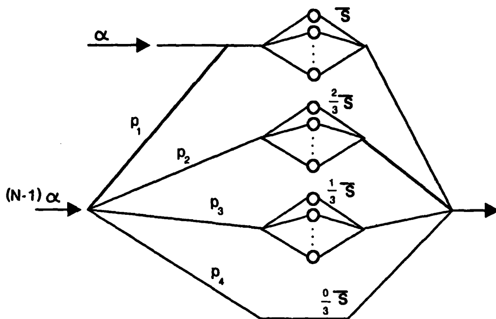
Figure 7-4: Multiple M/G/∞ queue model of done
