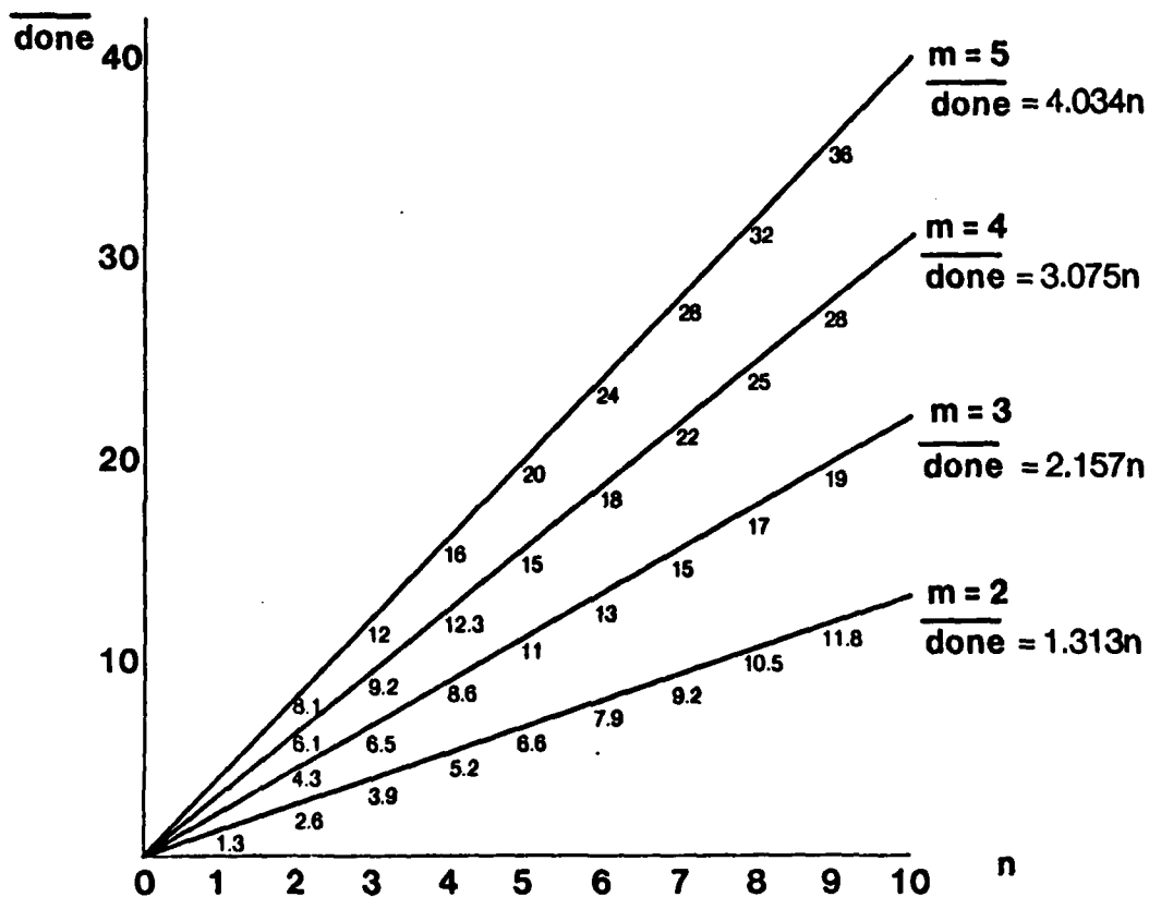
Figure 7-8: \overline{\text{done}} graphed as a function of n
