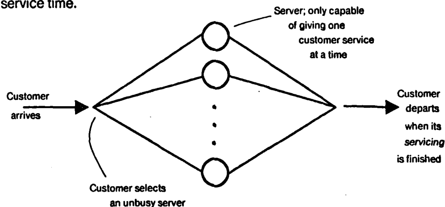
Figure 7-2: M/G/\infty queue
