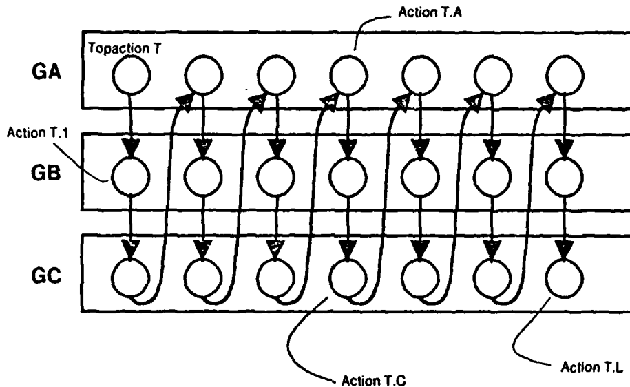
Figure 5-3: Recursion example
