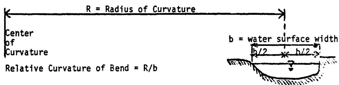
Figure 8. Definition Sketch for Relative Bend Curvature
