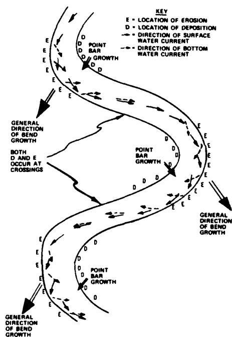
Figure 1. Migration of meander loop and cutoff development (adapted from Klingeman and Bradley 1976)
