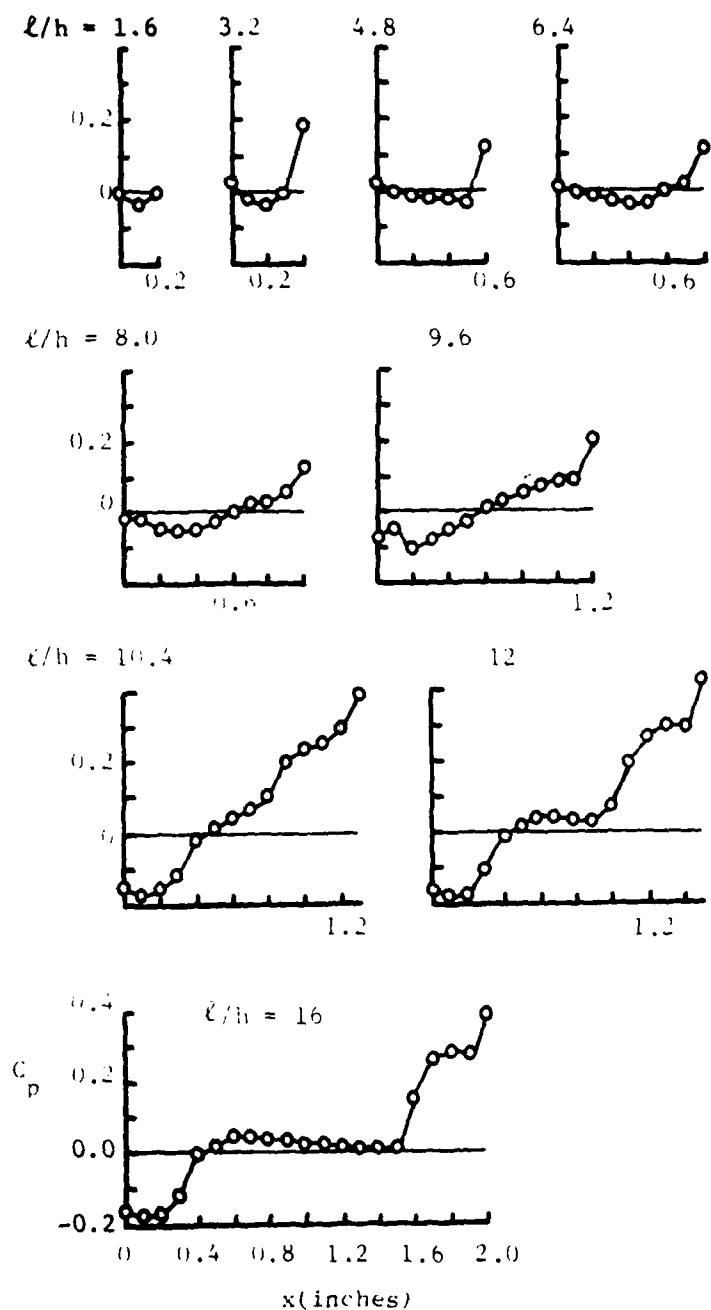
Figure 29 Pressure Distributions Along Floor of an Axisymmetric Cavity for M_\infty = 1.965 , h = 0.125 inches, (from Fig. 16, Ref. 39)
