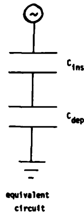
Fig. 16 Simple model for C-V analysis.
