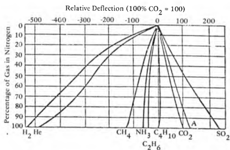
Figure A-2. Paramagnetic susceptibility of common gases.
