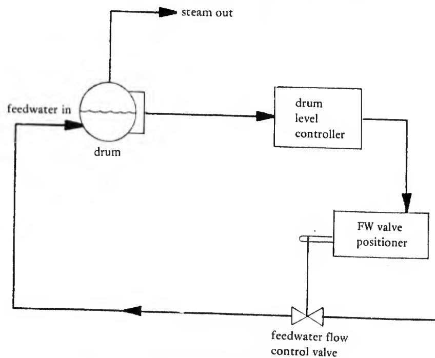
Figure 4. Single element feedwater control.
