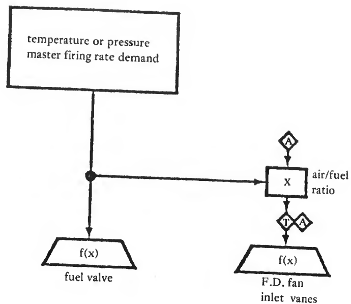
Figure 17. Parallel positioning system without O 2 trim – pneumatic or electric (Westinghouse-Hagan).
