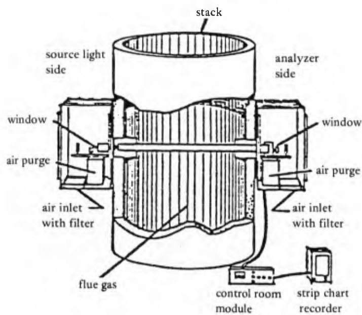
Figure A-6. Schematic arrangement of infrared carbon monoxide analyzer (Westinghouse-Hagan).
