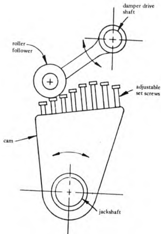
Figure 7. Adjustable jackshaft cam mechanism.
