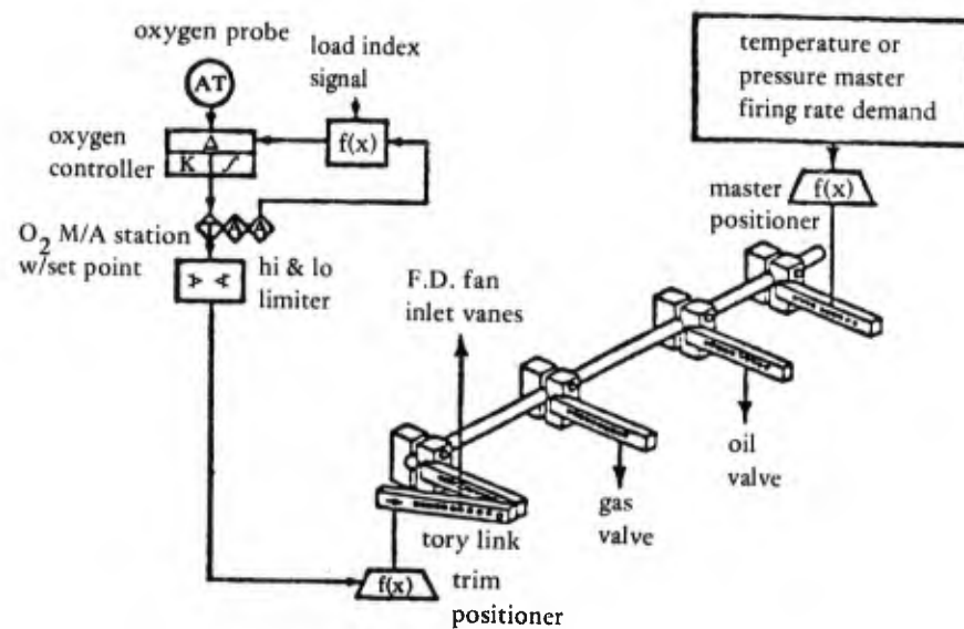
Figure 16. Jackshaft system with O_2 trim (Westinghouse-Hagan).
