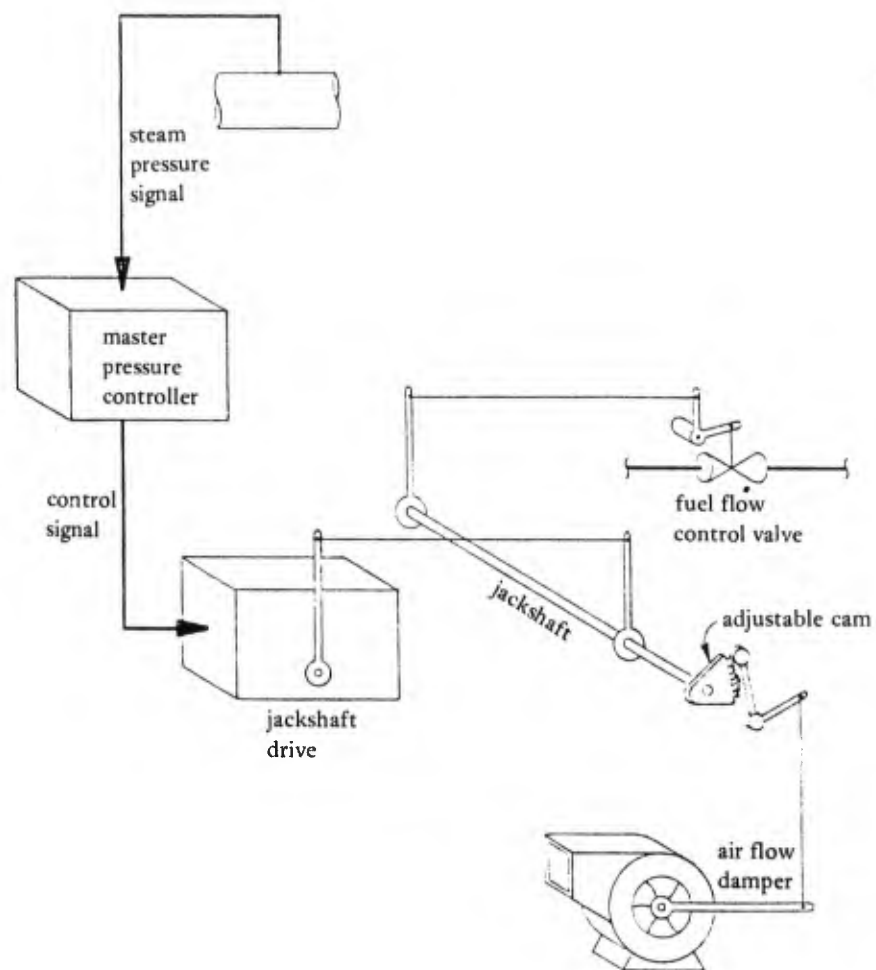
Figure 1. Jackshaft burner control system.
