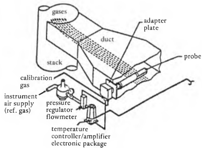
Figure A-5. Schematic arrangement of zirconium oxide O_2 analyzer (Westinghouse-Hagan).
