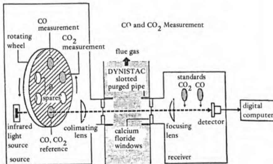
Figure A-7. Diagrammatic arrangement of infrared carbon monoxide analyzer (Measurex).
