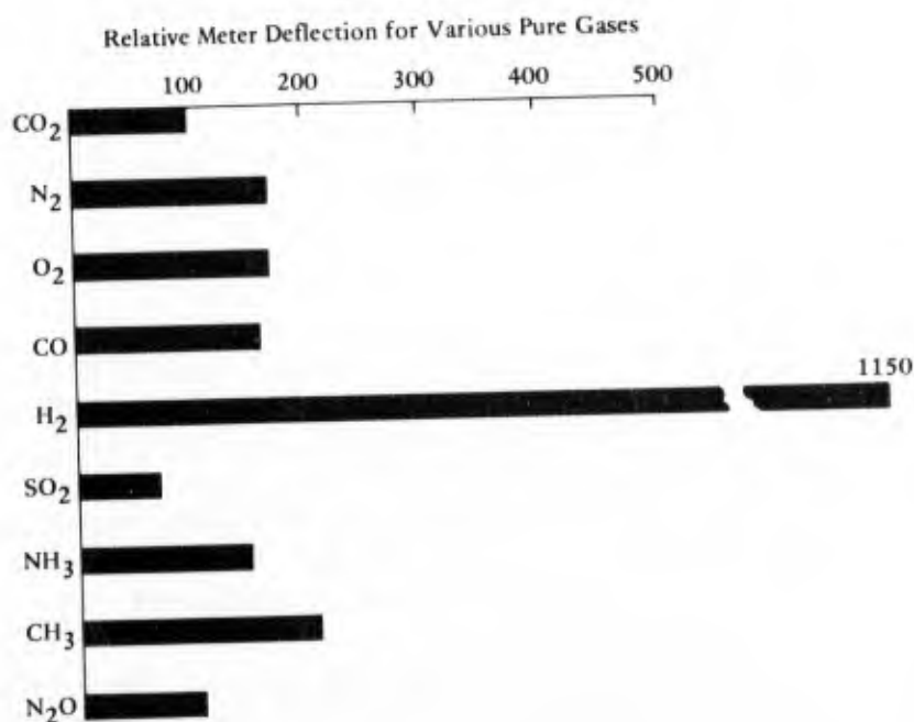
Figure A-1. Effect of passing different gas samples through thermal conductivity instrument.
