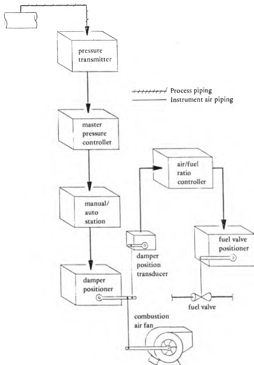
Figure 2. Series positioning control system (air leading fuel).
