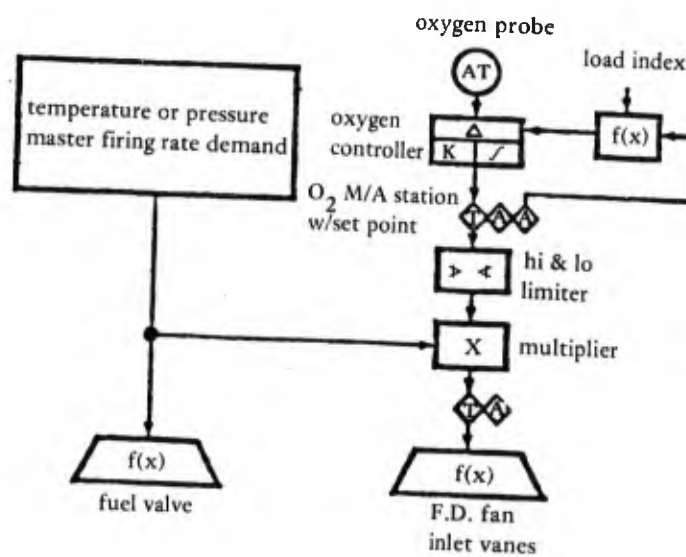
Figure 18. Parallel positioning system with O 2 trim – pneumatic or electric (Westinghouse-Hagan).
