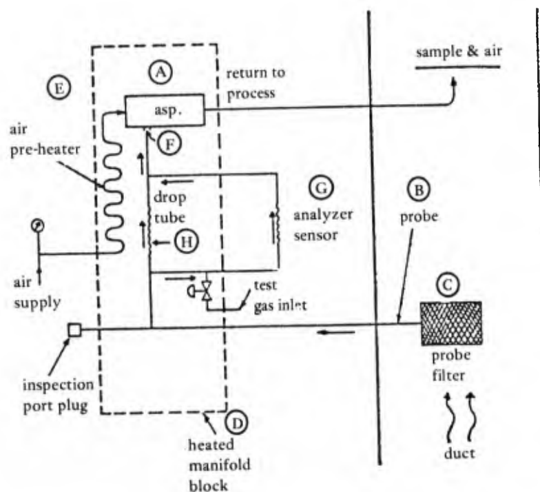
Figure A-4. Zirconium oxide O 2 analyzer sample flow diagram (B&W – Bailey).
