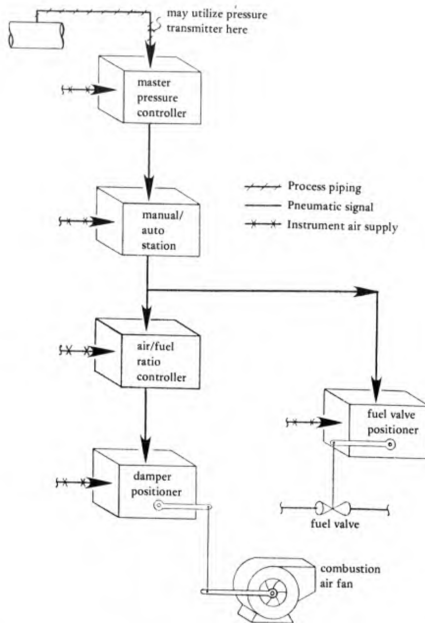
Figure 8. Parallel positioning control system (pneumatic).
