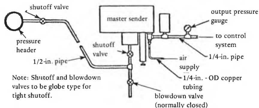
Figure 9. Master pressure controller instrument piping diagram.
