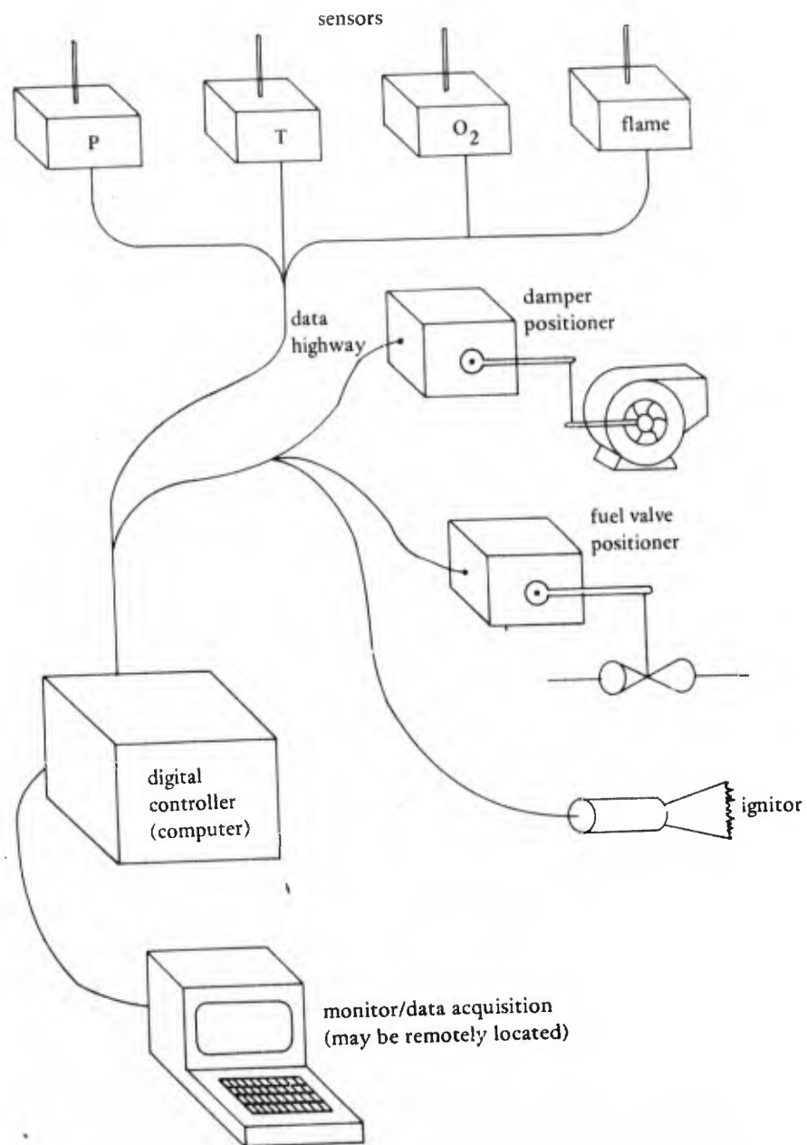
Figure 19. Digital control system.
