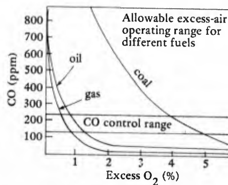
Figure 14. CO trim system operating point (from Ref 6).
