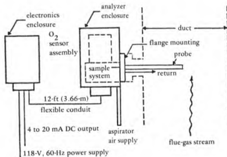
Figure A-3. Zirconium oxide O 2 analyzer block diagram (B&W – Bailey).
