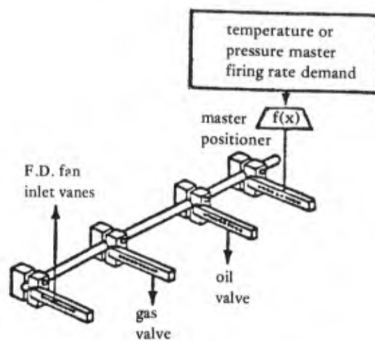
Figure 15. Jackshaft system without O_2 trim (Westinghouse-Hagan).
