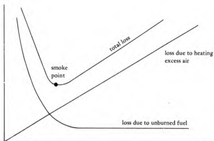
Figure 10. Boiler flue gas loss.
