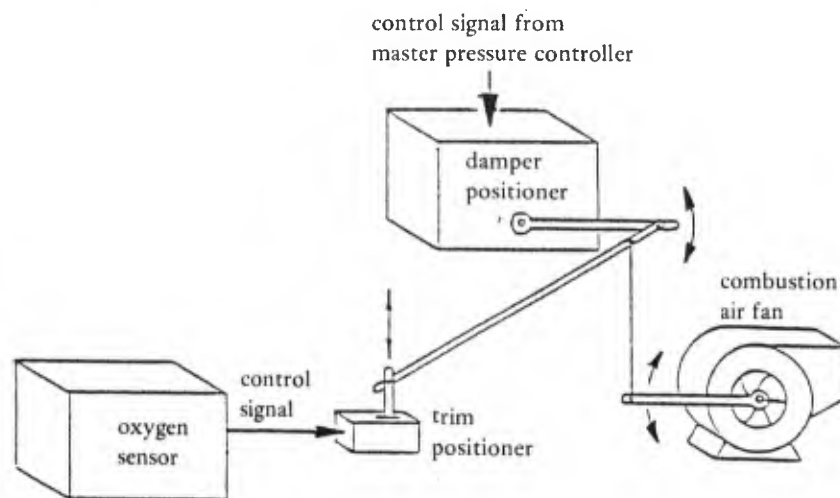
Figure 11. Oxygen trim system.
