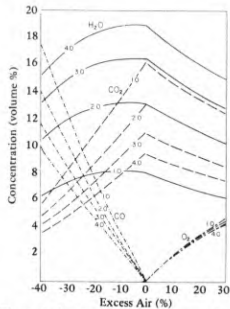
Figure 12. Theoretical composition of flue gases for several HC ratios. Hydrogen/carbon ratios: natural gas = 4, no. 2 oil = 1.7, no. 6 oil = 1.3, coal = 0.7 (from Ref 5).
