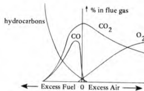
Figure 13. Variation of flue gas constituents with excess air level.
