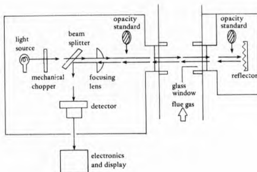
Figure A-8. Smoke (opacity) analyzer (Measurex).
