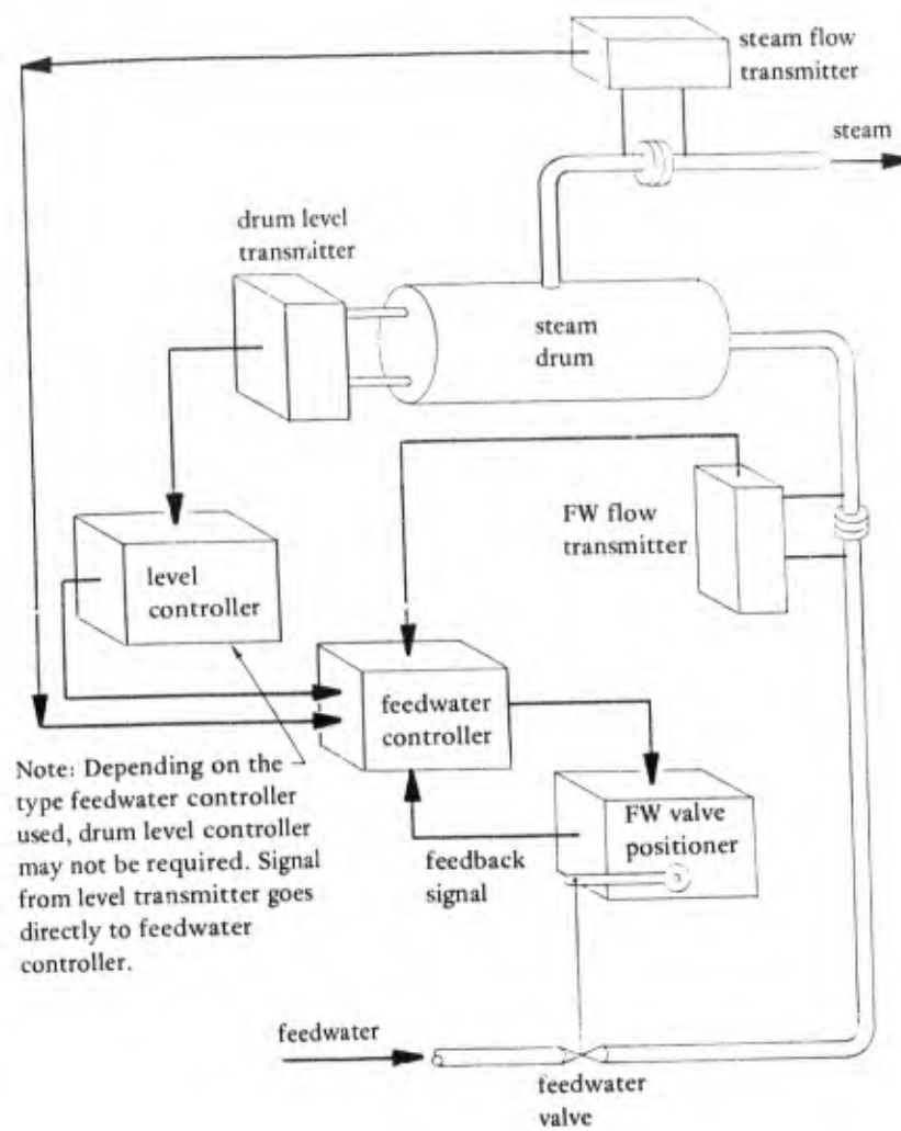
Figure 5. Three-element feedwater control.
