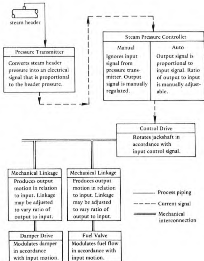
Figure 6. Functional schematic diagram of jackshaft system.
