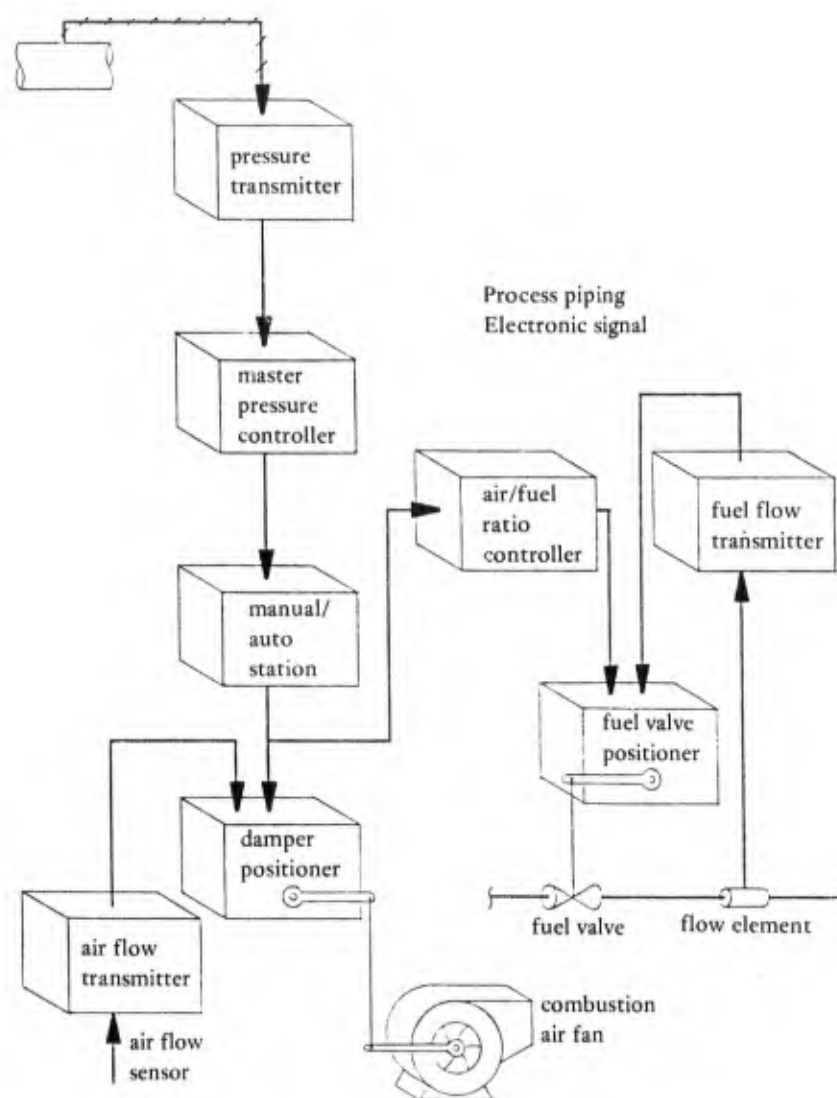
Figure 3. Metering control system.
