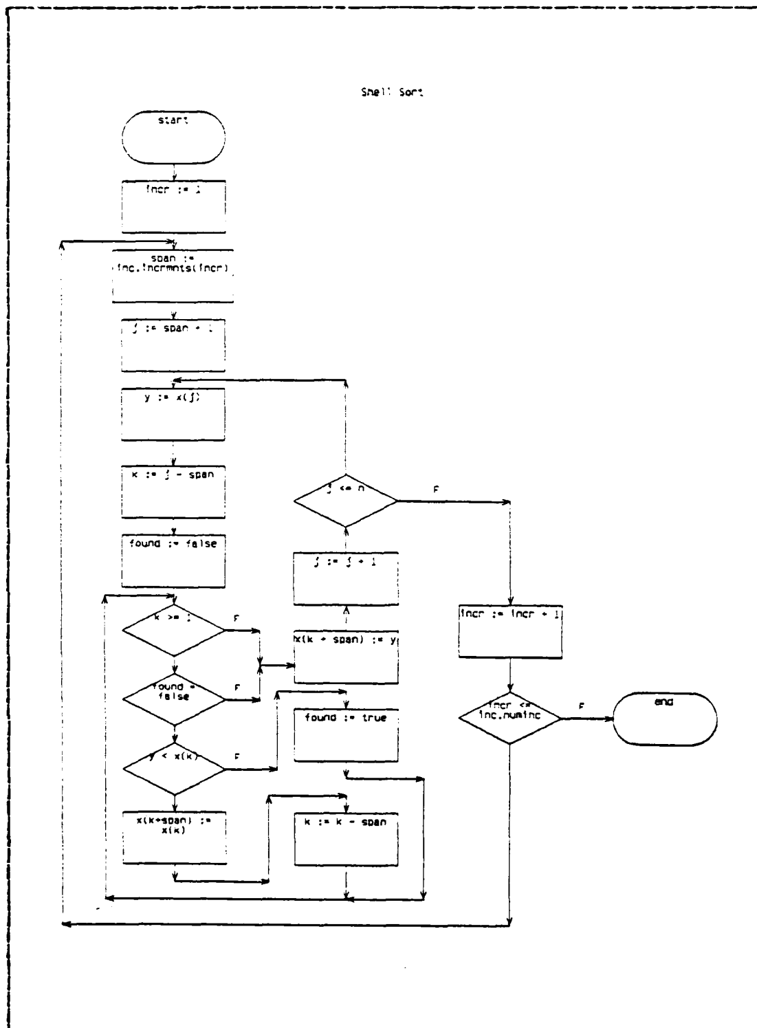
Figure 4.9 Flow Diagram of Shell Sort
