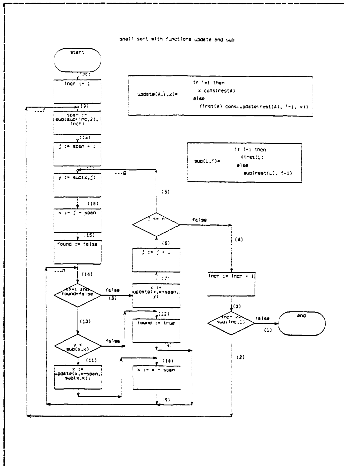
Figure 4.10 Shell Sort with "sub" and "update"
