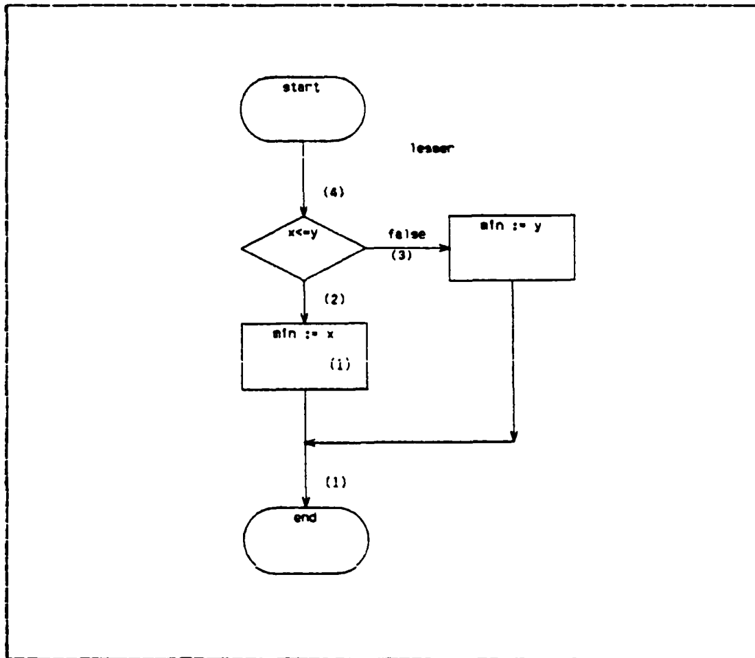
Figure 4.3 Flowchart of "lesser"
