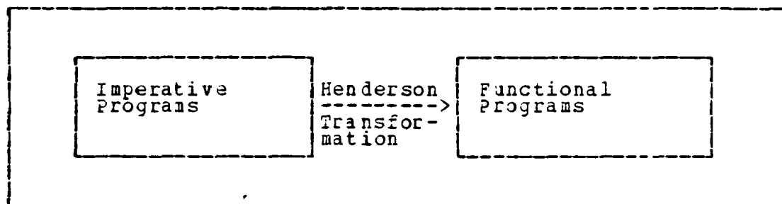
Figure 4.1 Program Transformation
