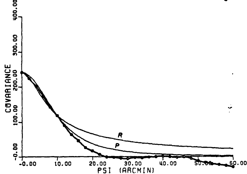
Figure 16 Degree variances, power spectrum and covariance function for free-air gravity anomalies in a 2°x2° area of Ohio. See text for detailed figure explanation.
