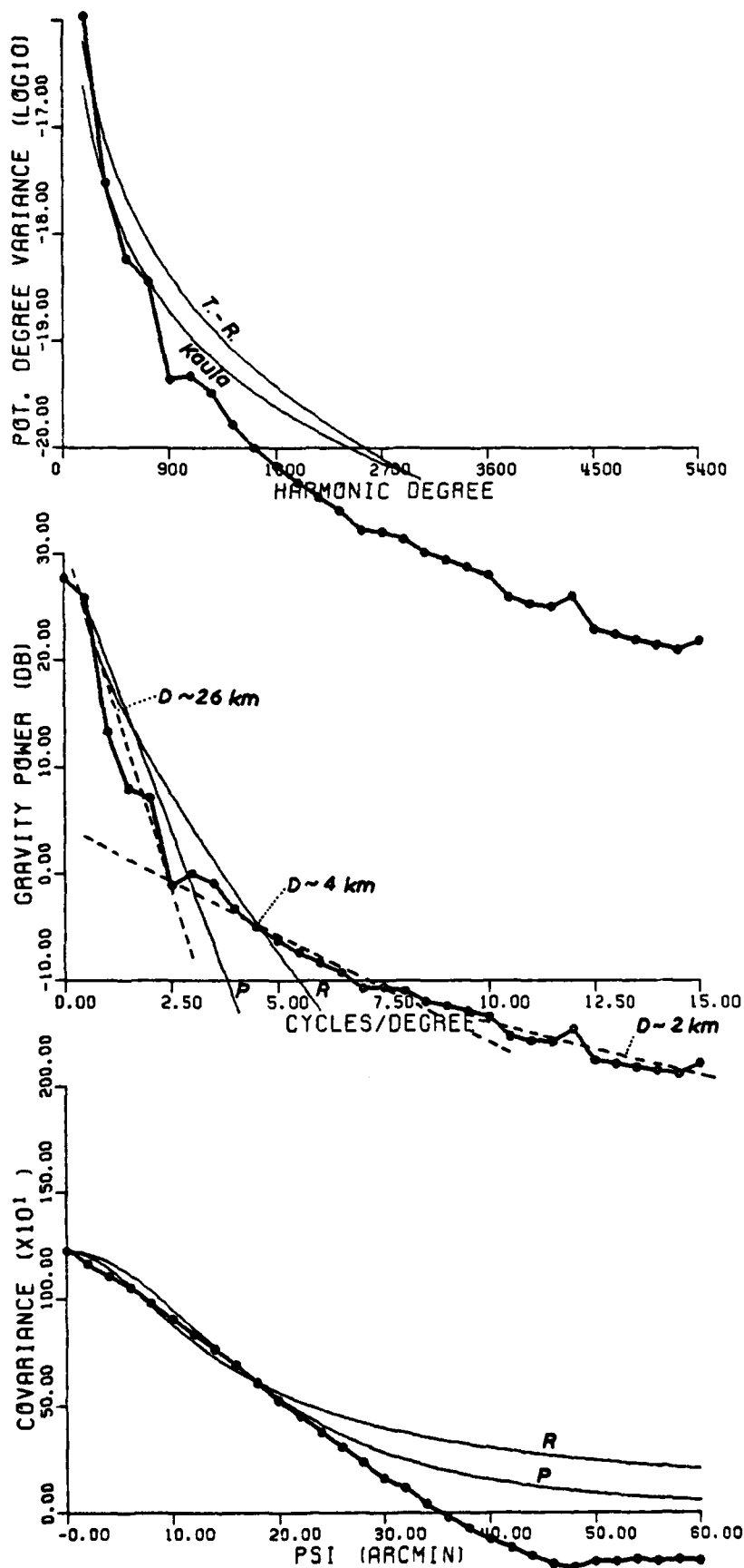
Figure 18 Degree-variances, power spectrum and covariance function for residual Bouguer (RTM) anomalies in a 2°x 2° area of California.
