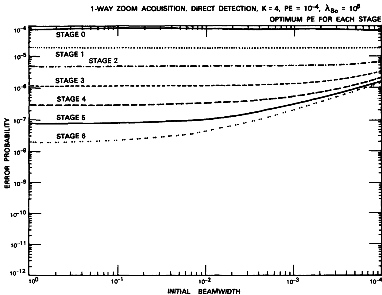
Fig. 4.6. Acquisition with zooming receiver, background and quantum noise limited direct detection, \lambda_{B0} = 10^6 : (b) optimal partition of PE, 1-way zooming strategy.
