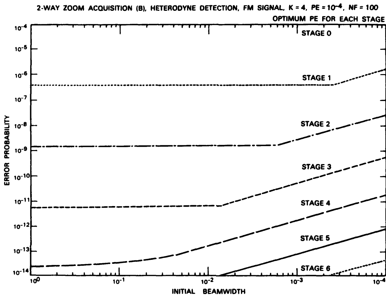
Fig. 4.3. Acquisition with zooming receiver, heterodyne detection, simultaneous frequency acquisition: (f) optimal partition of PE, 2-way zooming strategy (B).
