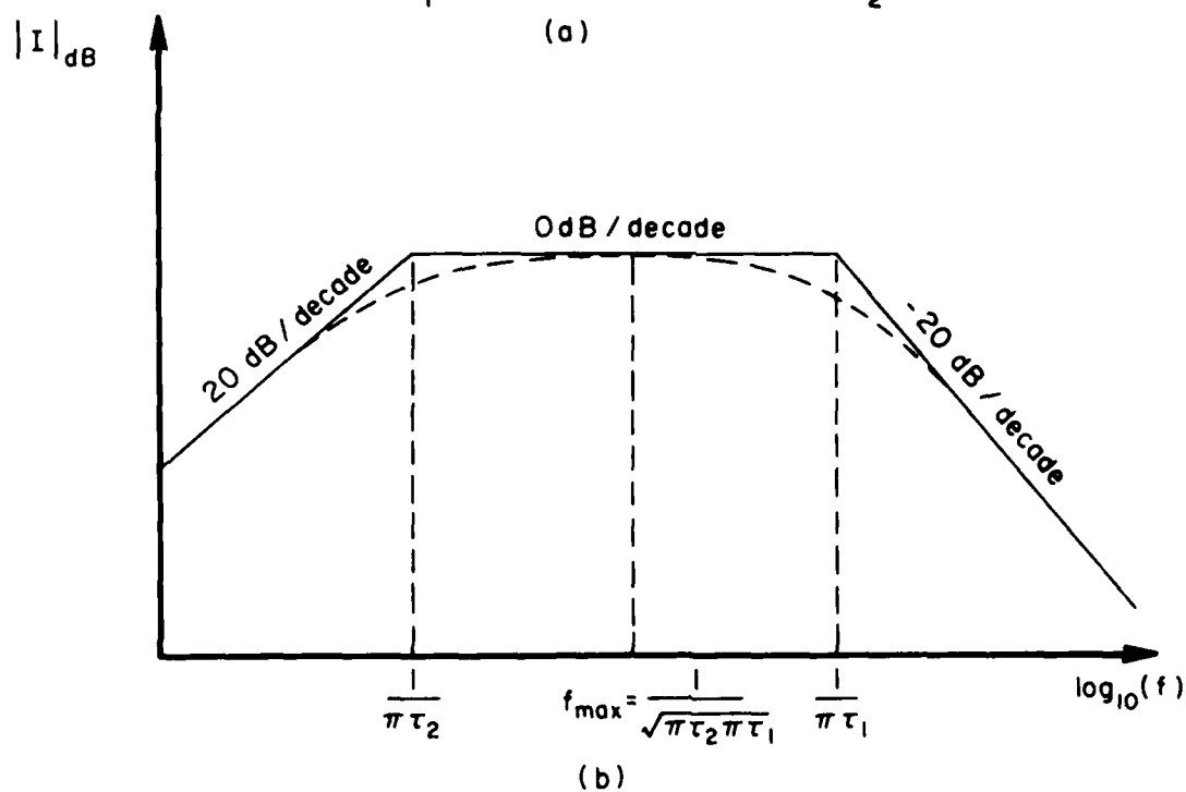
Fig. 3-2. Bounding the frequency response.
