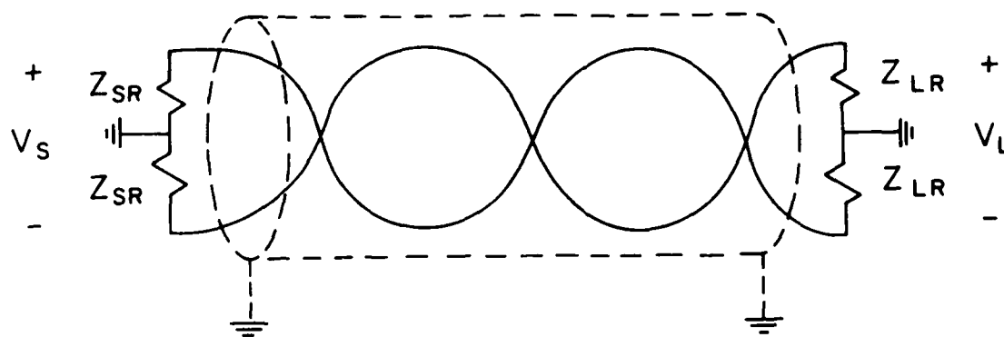
Fig. 2-15. The receptor circuit wire types.
