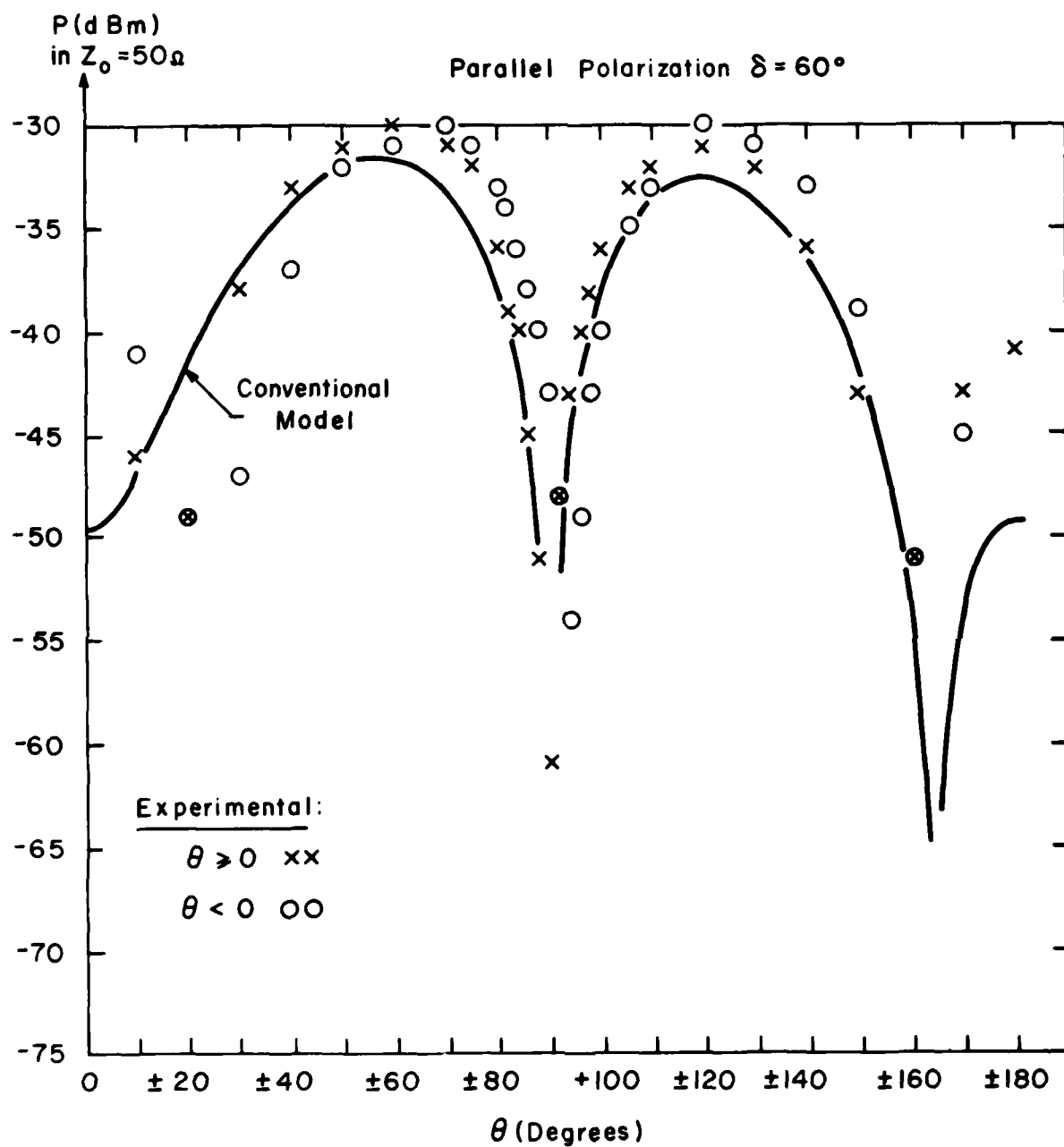
Fig. 3-5. Predictions of the model for parallel polarization and L = 25 cm, k = 5 mm, f = 1.2 GHz, \delta = 60^\circ .
