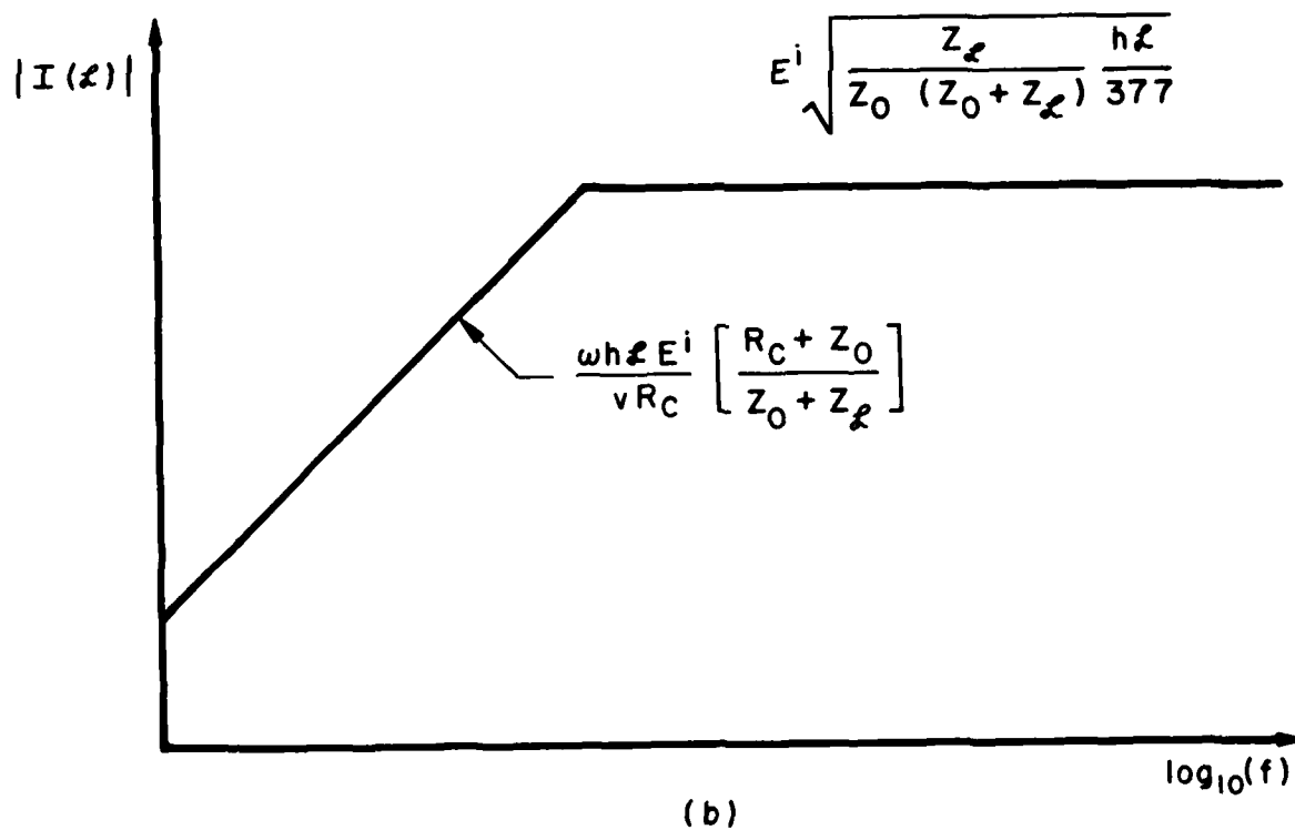
Fig. 3-8. Bounds on the induced currents.
