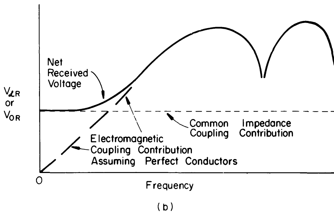
Fig. 2-16. Common impedance coupling.
