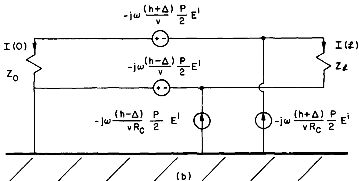
Fig. 3-9. The unbalanced, twisted pair model.
