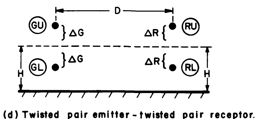
Fig. B-1. The cross-sectional configurations.
