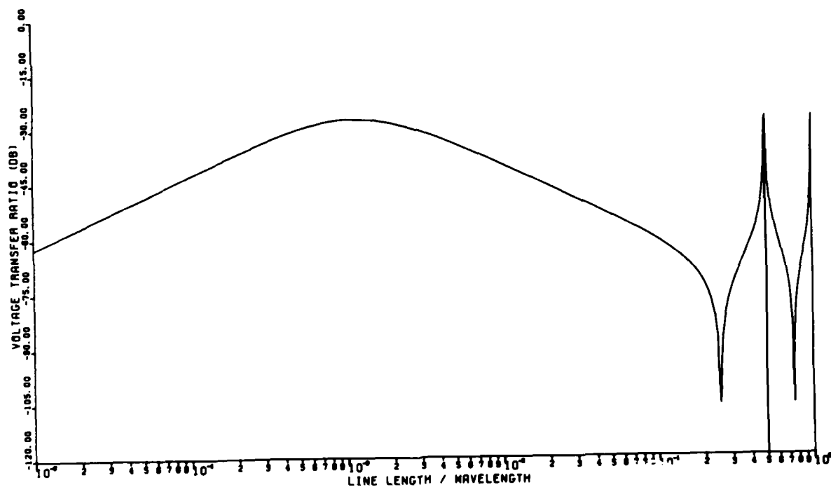
Fig. 2-7. Frequency response plots for the example.
