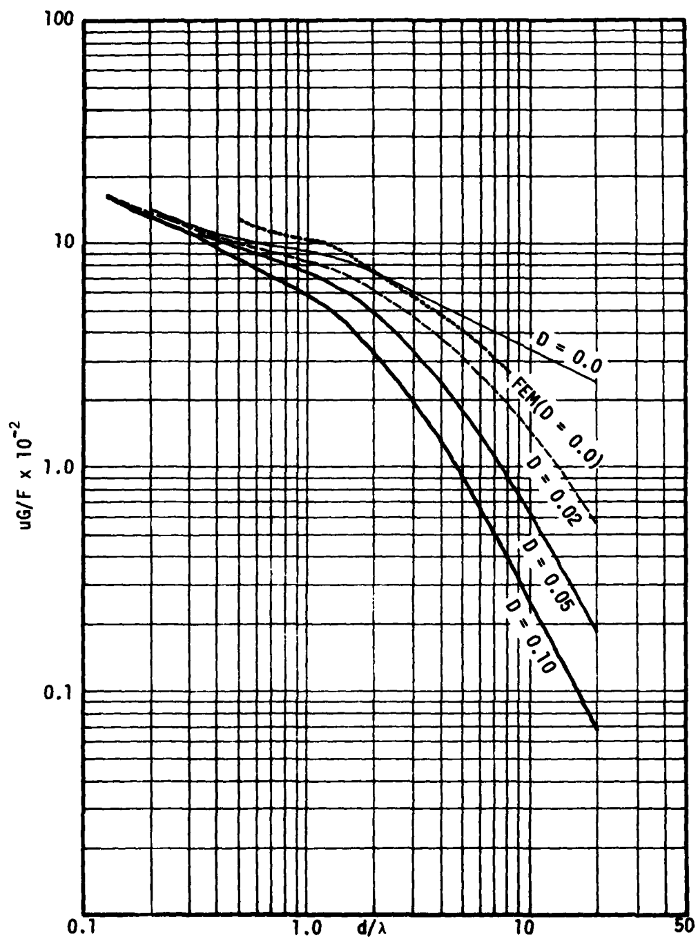
Figure 6.10 - 2-D Attenuation, Free Field
