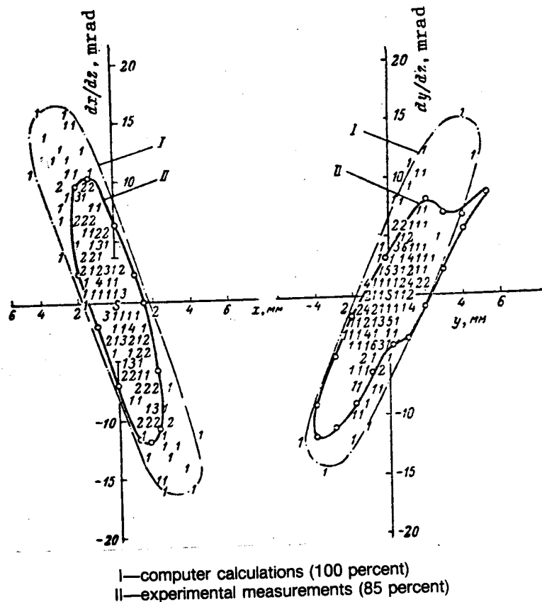
Fig. 24—Beam emittance at the output of the URAL-15 accelerator [31]
