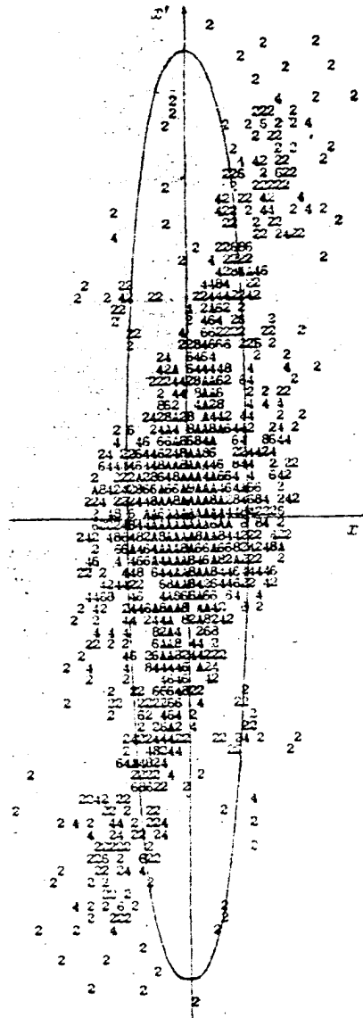
Fig. 34—Phase diagram of a bunched beam in the x, x' plane [44]. Beam current is 75 mA. The ellipse represents phase space occupied by an unbunched beam.
