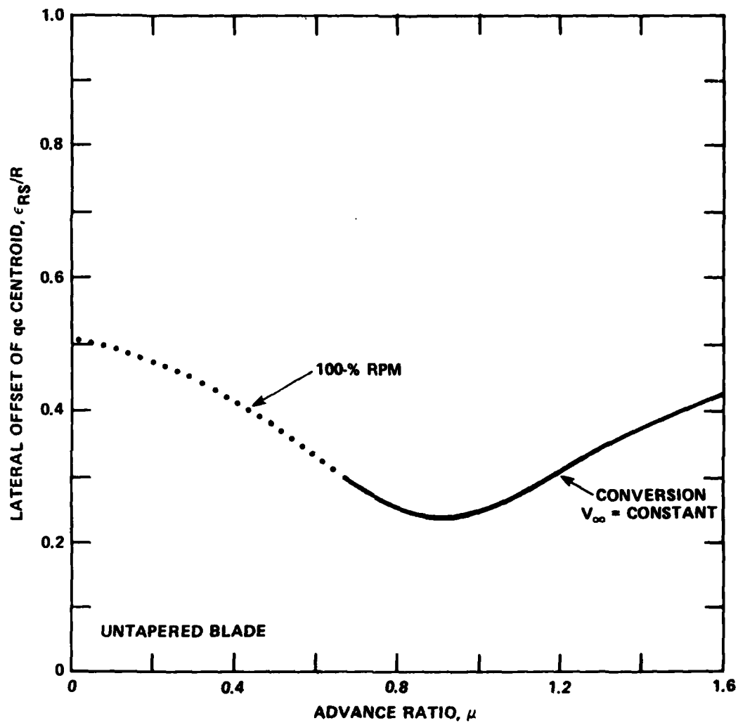
Figure 7 - Characteristics of Retreating Side Roll Moment Arm
