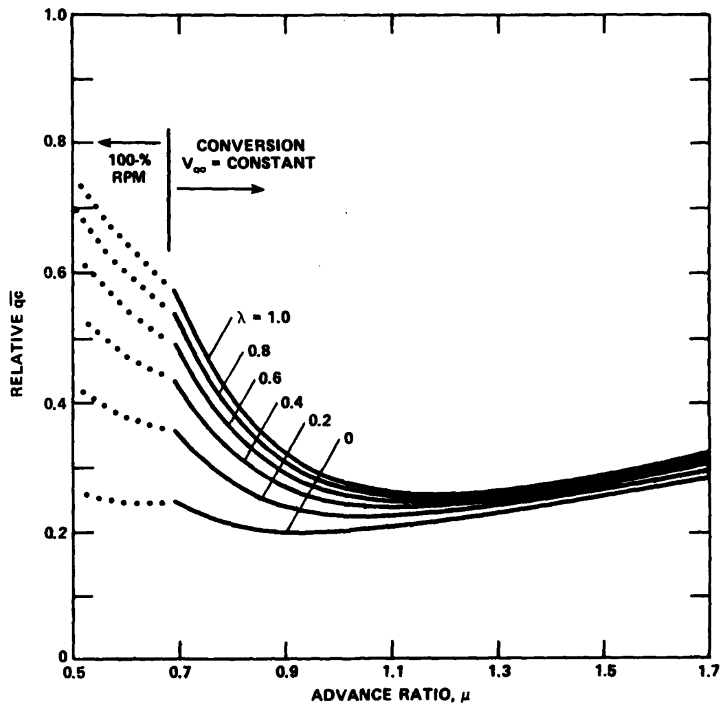
Figure 6 - Effect of Blade Planform on Critical Condition
