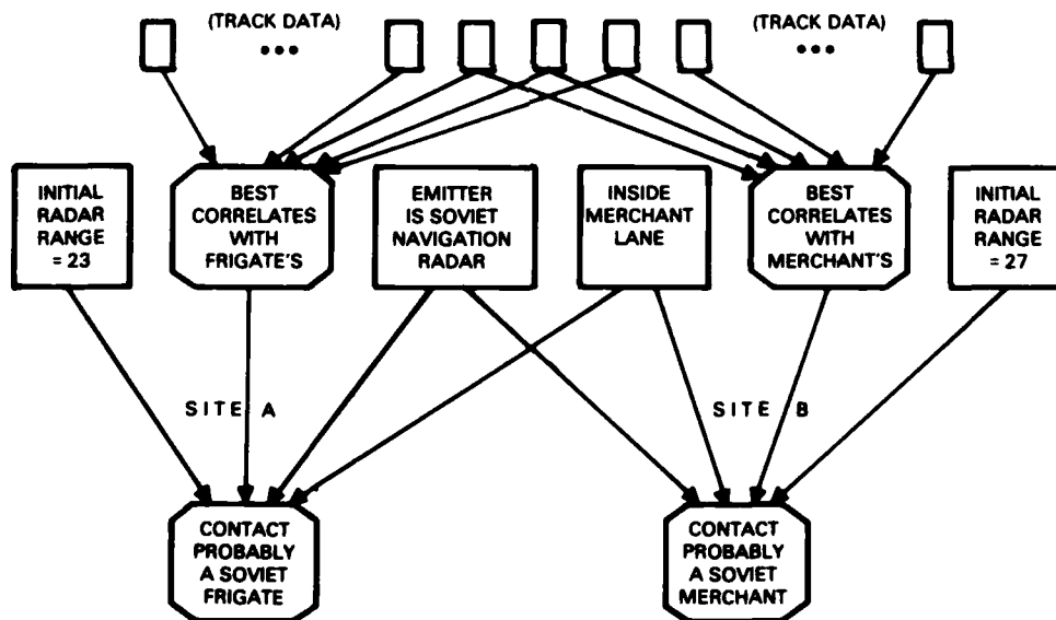
Figure 2. An example of different units reaching different conclusions. (Rectangles represent observed data; other blocks represent conclusions.)
