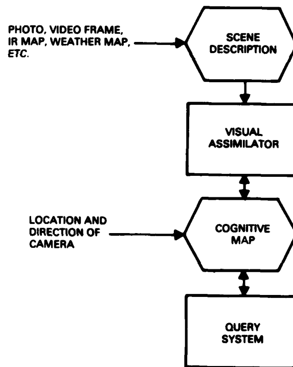
Figure 4. Generalized MERCATOR structure.
