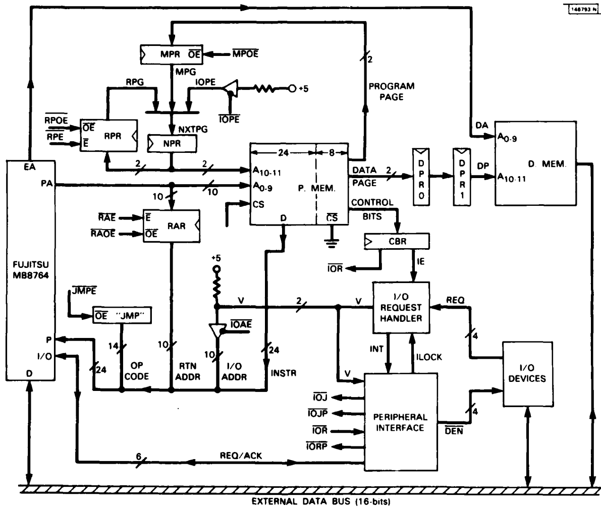
Fig. 6. Component level implementation of MB8764-based speech processor.
