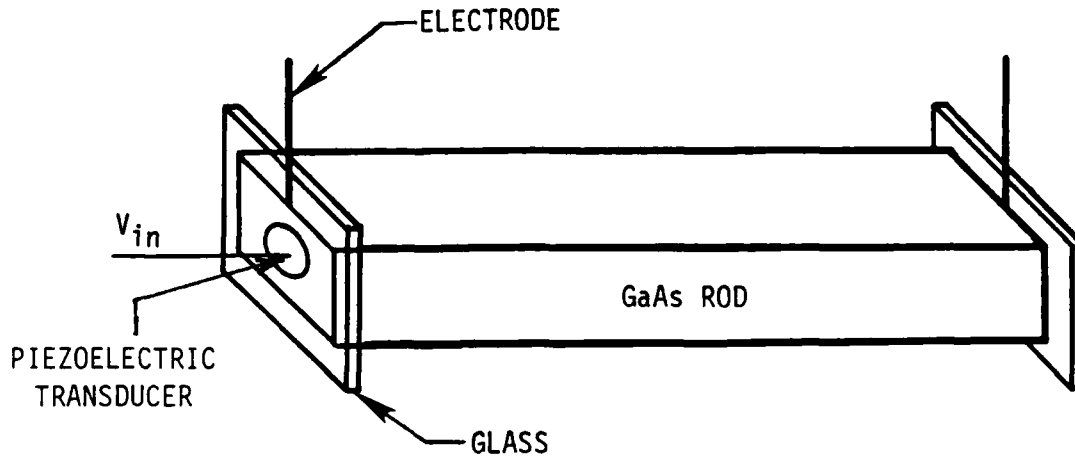
FIGURE 35. SEMI-CONDUCTOR GRATING
