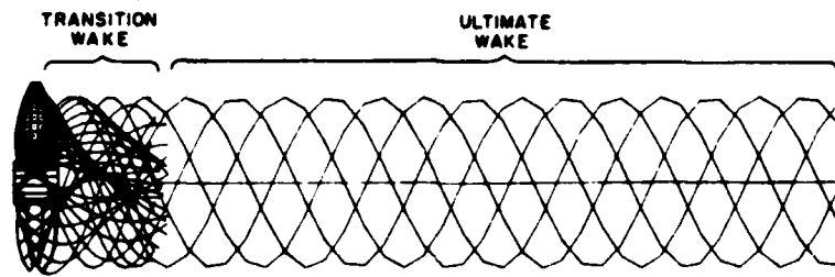
Figure 4 - Trailing Wake Geometry after Wake Alignment
