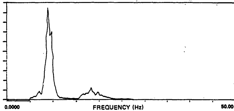
DISPLACEMENT SPECTRUM
