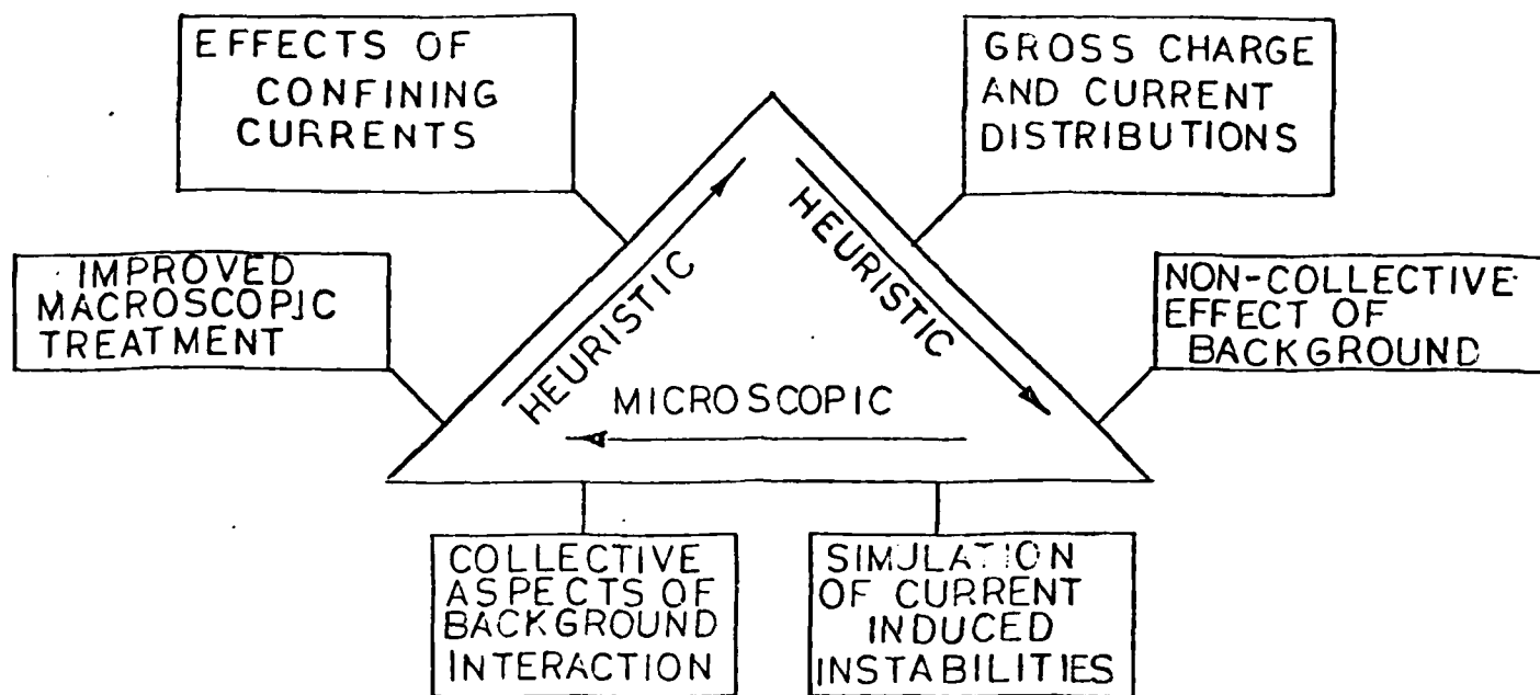
FIGURE 4. A NUMERICAL STUDY COMBINING HEURISTIC, MACROSCOPIC MODELLING WITH MICROSCOPIC, PARTICLE-IN-CELL SIMULATIONS
