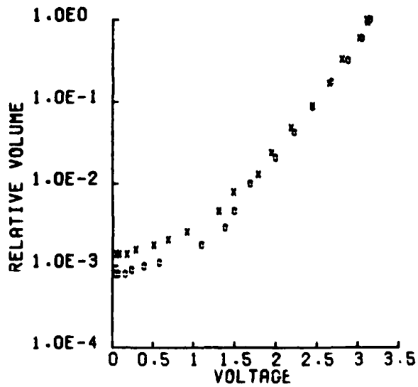
Figure 4. Graph of normalized aerosol volume and flame photometer voltage: Experiments 3 and 4.
