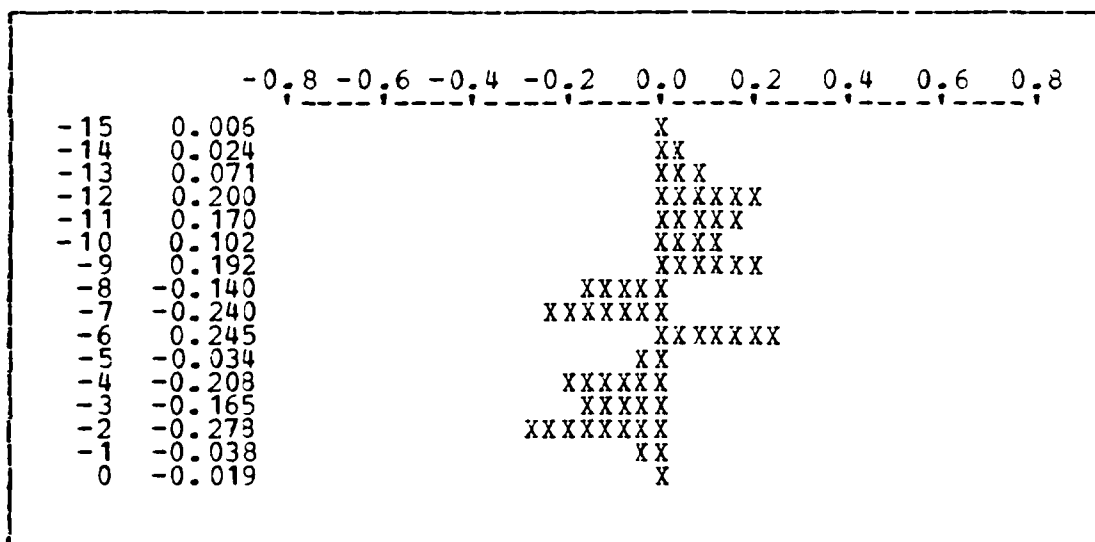
Figure 3.7 CROSS CORRELATION FOR OS RATING.
