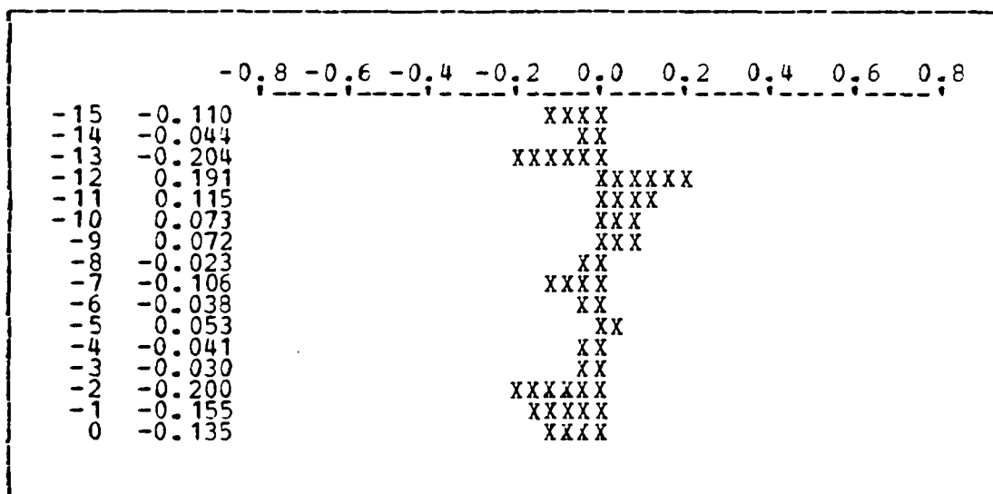
Figure 3.5 CROSS CORRELATION FOR YN RATING.
