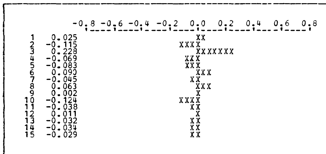
Figure 3.2 AUTOCORRELATION FUNCTION FOR UNEMPLOYMENT DATA.
