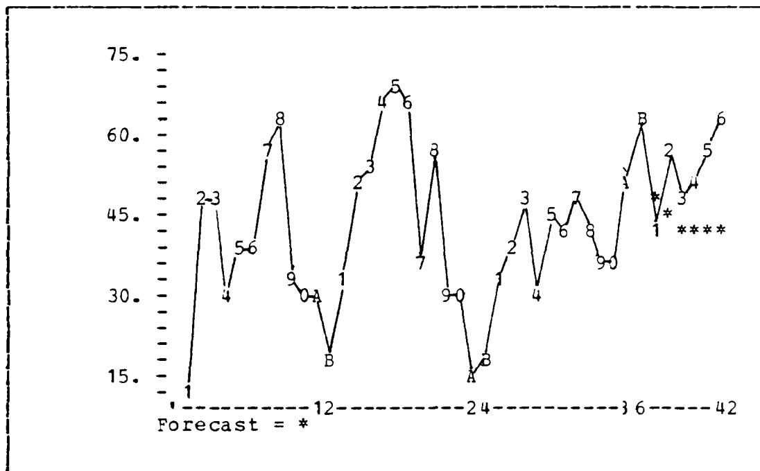
Figure 2.20 PLOT OF UNIVARIATE MODEL FOR BT RATING.
