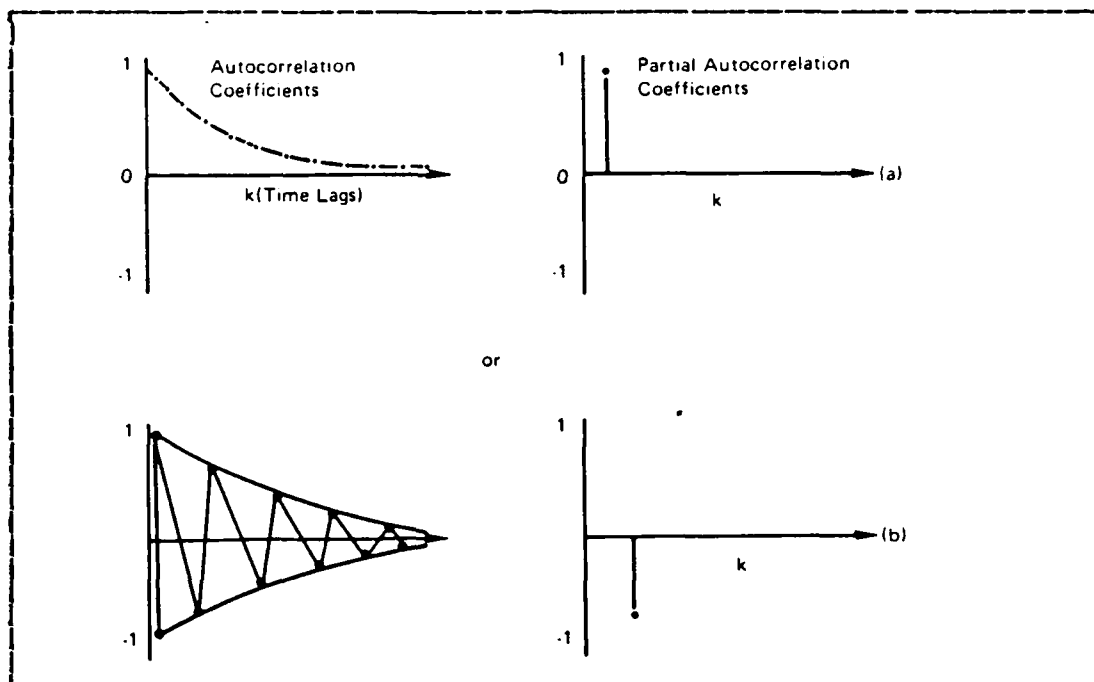
Figure B.4 TYPICAL FORM OF AR1 MODEL ACF AND PACF.
