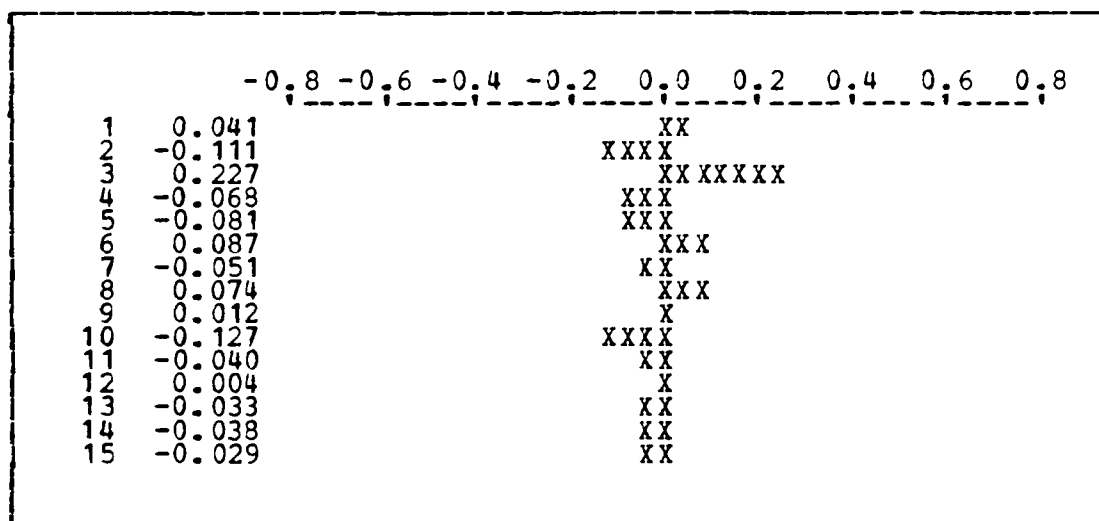
Figure 3.4 AUTOCORRELATION OF RESIDUALS FOR UNEMPLOYMENT MODEL.
