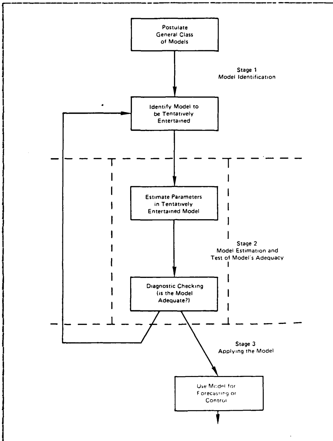
Figure B.1 THE BOX-JENKINS METHODOLOGY.
