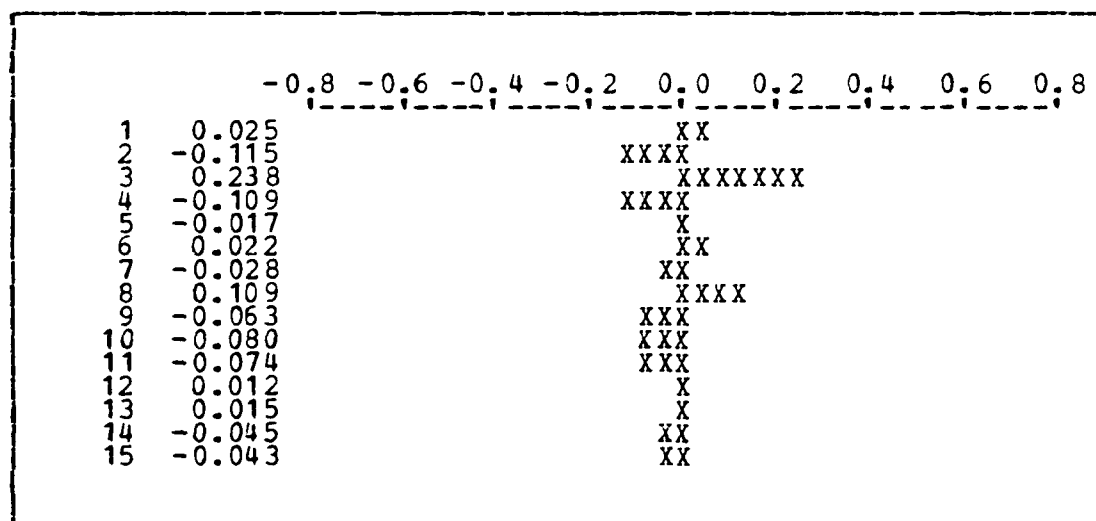
Figure 3.3 PARTIAL AUTOCORRELATIONS FOR UNEMPLOYMENT DATA.
