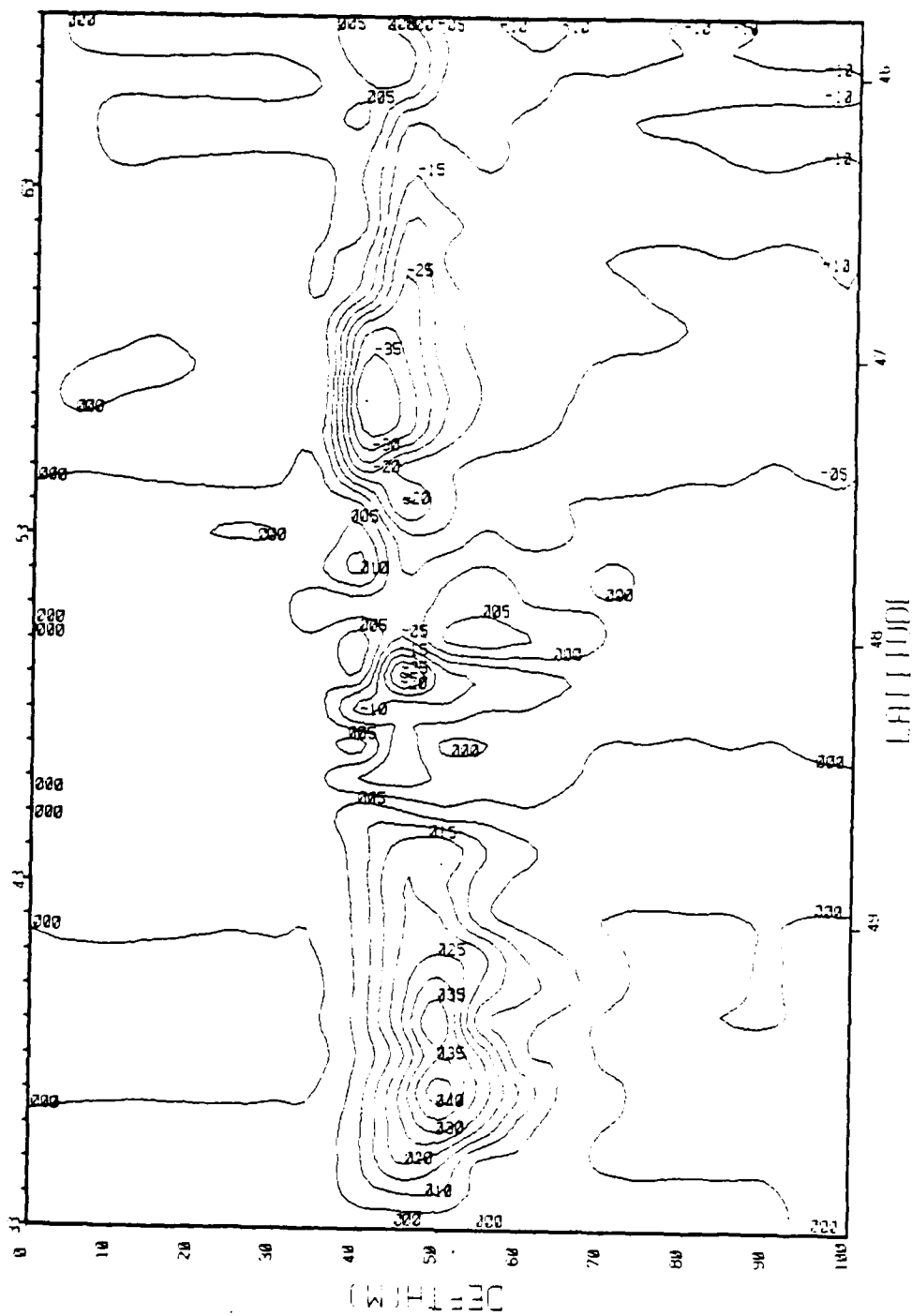
Figure 16. Same as Figure 15 but for points 33-68 and section 2.
