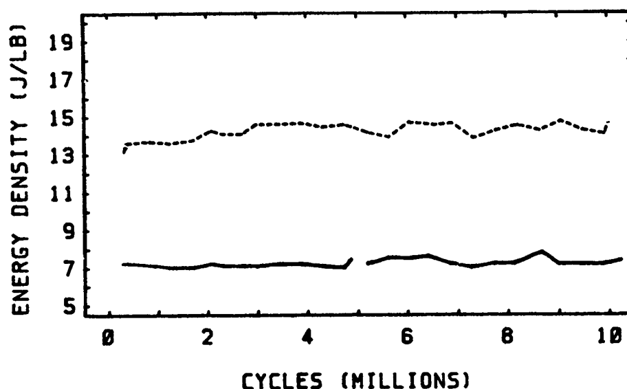
— 0.013% - - - - - 0.025% ENERGY DENSITY VERSUS CYCLES FIGURE 5-5
