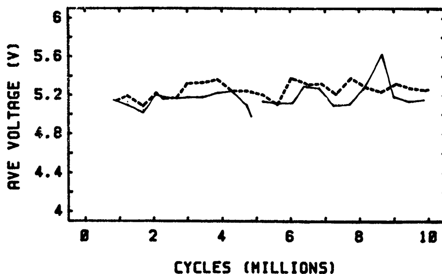
— 0.013% - - - - - 0.025% AVERAGE BATTERY VOLTAGE VERSUS CYCLES FIGURE 5-4
