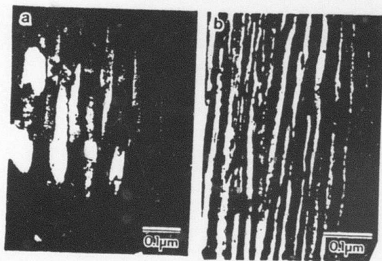
Fig. 1. Eutectic structures of \alpha -Cr and \beta -NiAl solidified at (a) 0.09 cm/s and (b) 0.8 cm/s with spacings of \sim 80 nm and \sim 20 nm respectively. TEM.
