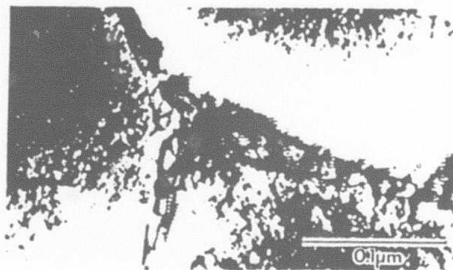
Fig. 2. Intercellular region in alloy solidified at 12 cm/s. TEM.
