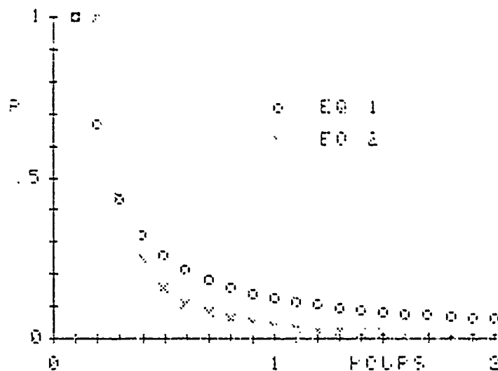
Figure 1. Plots of p as a function of t based on Equations 1 and 2 for u_M = 20 knots, r_C = 2 nautical miles and M = 4 weapons.
