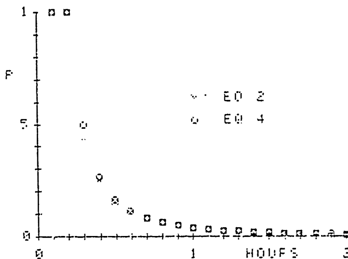
Figure 2. Plots of p as a function of t based on Equations 2 and 4 for u_M = 20 knots, r_O and r_C = 2 nautical miles and n = 4 weapons.
