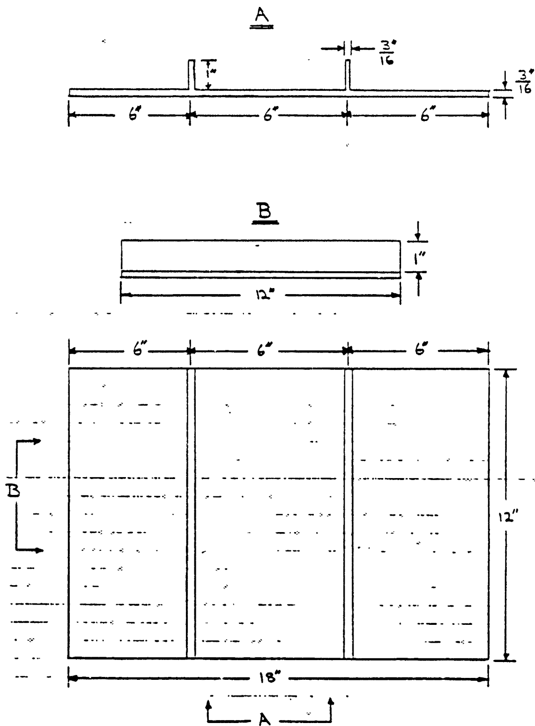
Fig. 2.1 Test Panel
