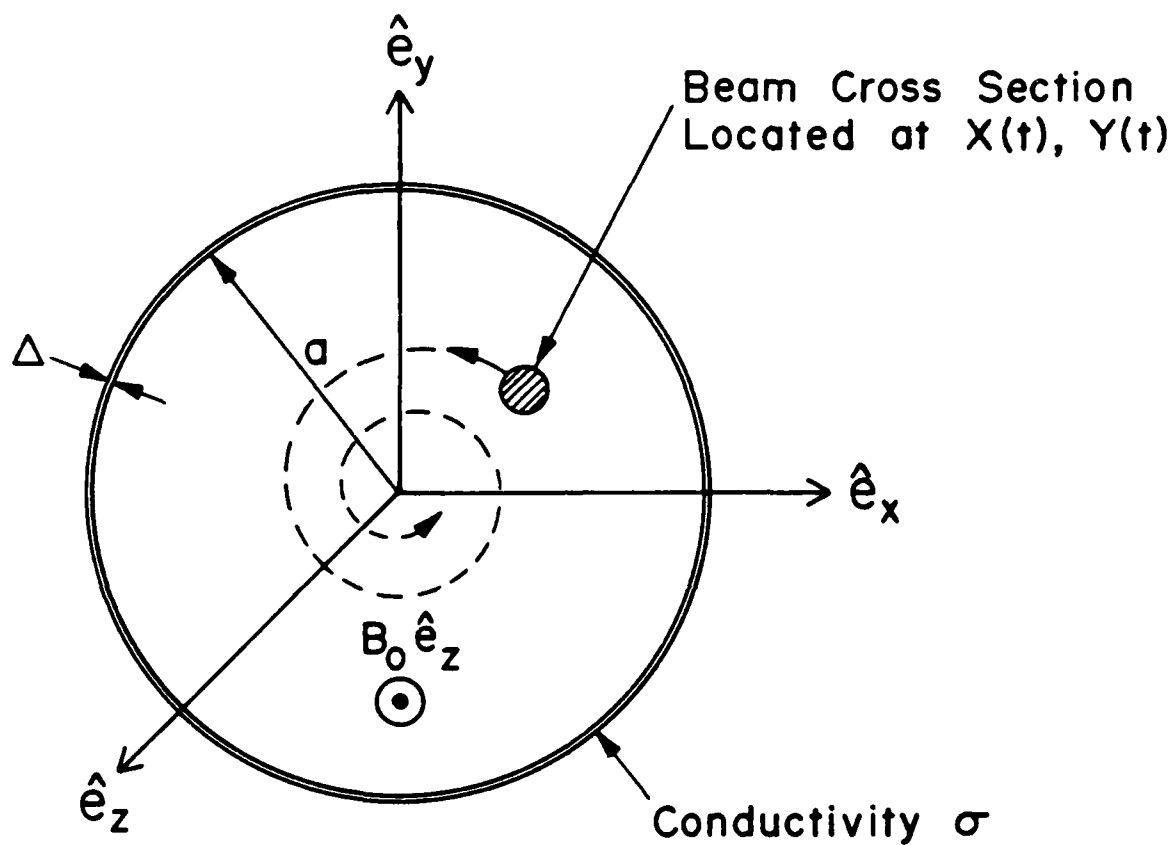
Figure 2 Model of cross section of rebatron chamber showing the tranverse location of the electron beam. The beam transverse dynamics is influenced by the torsatron field, axial magnetic field and induced fields.
