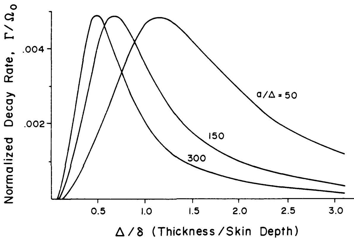
Figure 3 Shows the decay rate for the beam centroid as a function of \Delta/\delta for a/\Delta = 50, 150, 300 , \epsilon_o = 0.2 , \epsilon_w = 0.25 , \epsilon_s = 0.02 and \gamma_o = 5 .
