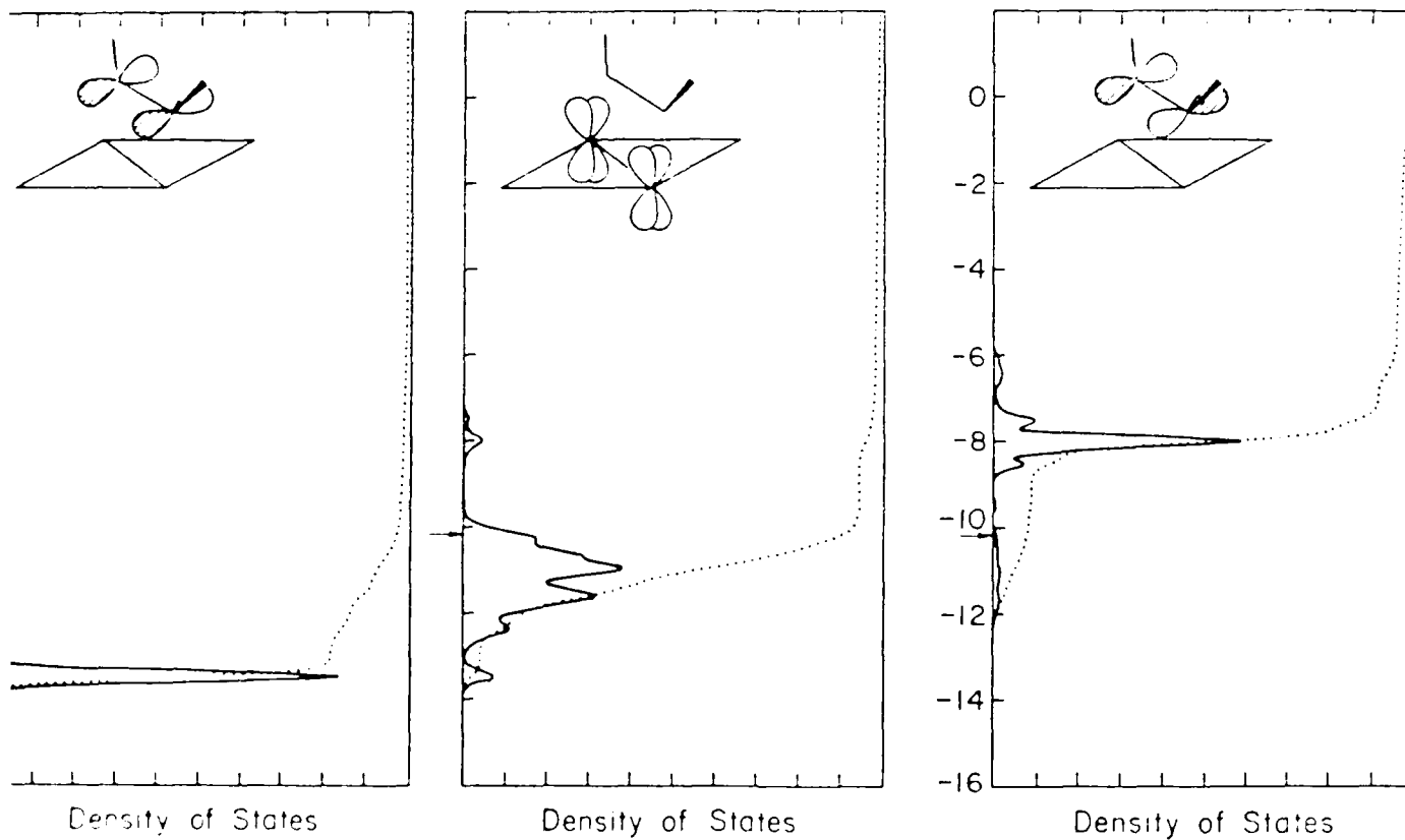
Figure 6. From left to right: contributions of \pi , yz ( \text{Pt}_1 , \text{Pt}_2 ) and \pi^* to the DOS of the \text{C}_2\text{H}_2/\text{Pt}(111) system in the 2-fold geometry. The curves are magnified by a factor of 10.
