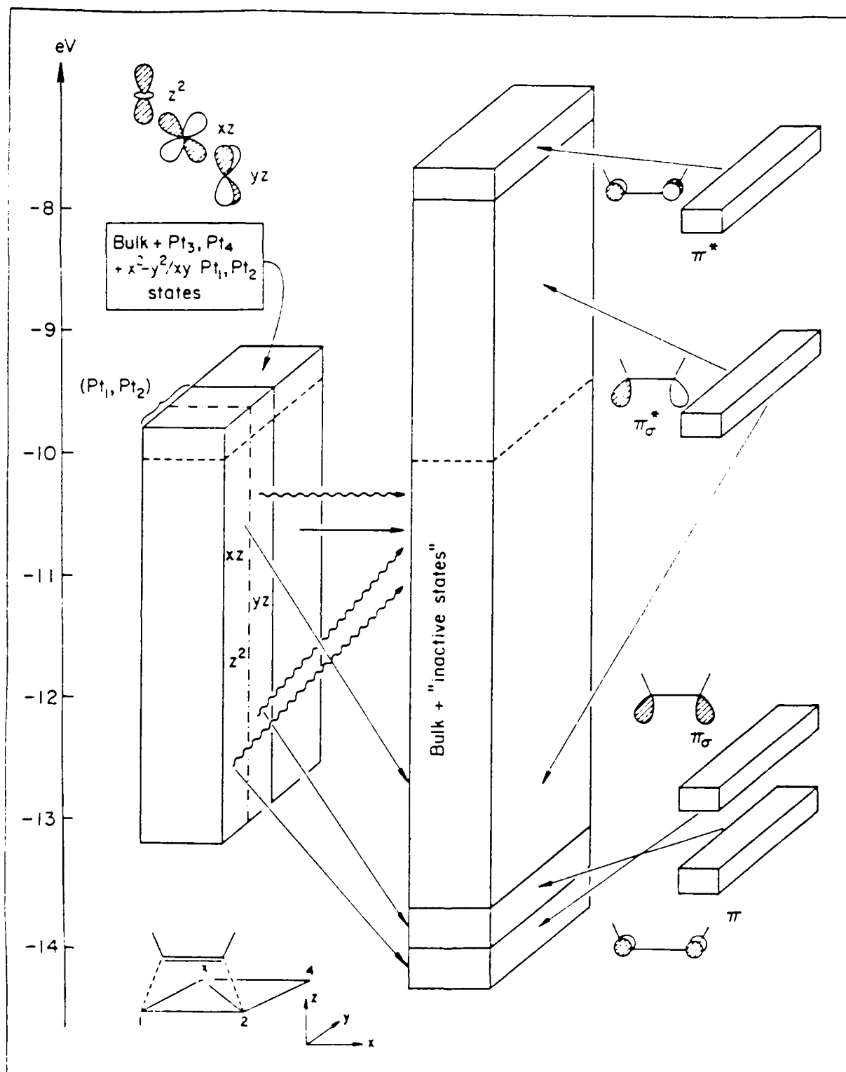
Figure 8. A generalized interaction diagram for \text{C}_2\text{H}_2 on \text{Pt}(111) in the 2-fold geometry.
