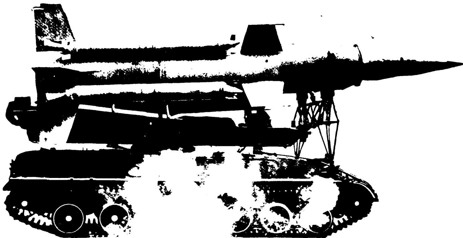
SA-4 ON TRACKED CHASSIS WHICH ALSO SERVES AS FIRING PLATFORM
