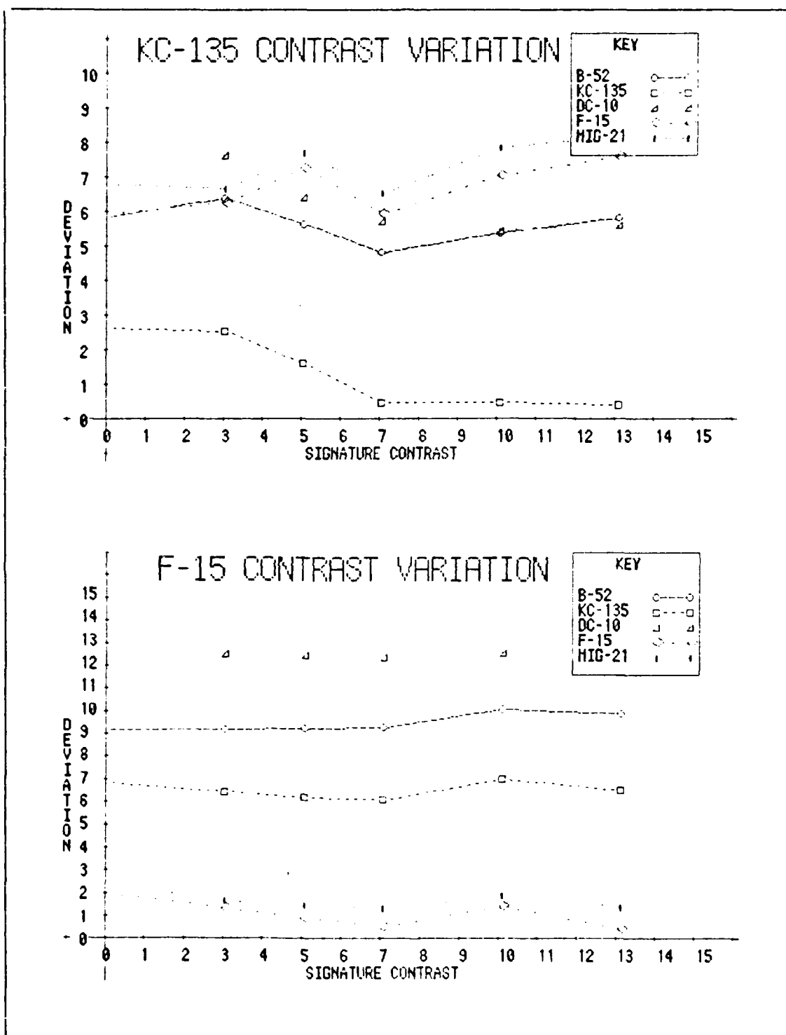
Figure 6-4. Effects of Variable Target Energy on Target Extraction Performance (Top:KC-135, Bot: F-15)
