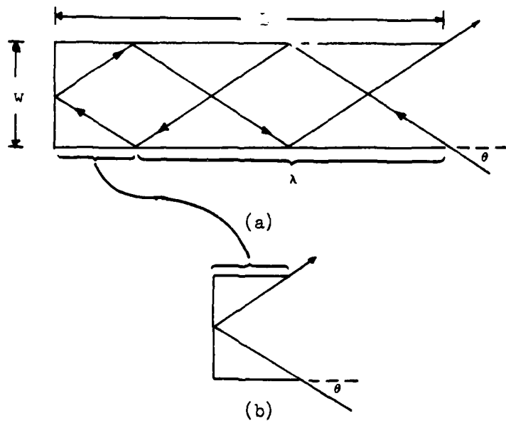
Fig. 2-2. Wavelength of a Two-Dimensional Cavity
