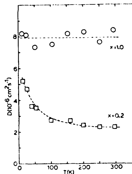
Fig. 2. Temperature dependence of the exciton diffusion coefficient for two samples.
