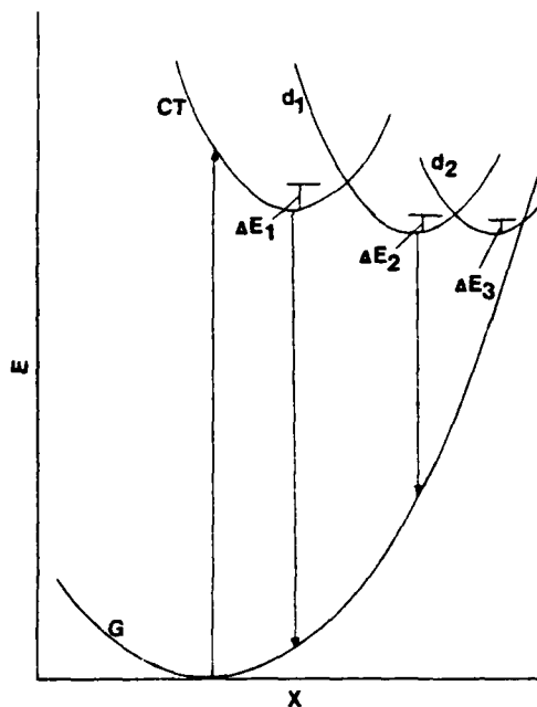
FIG. 10. Simplified single configuration coordinate model for interpreting the experimental results.
