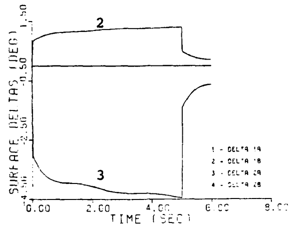
Fig. G-5(e). Control Surface Deflections for Roll Rate Command, Flight Condition 3--CSC Mode 5
