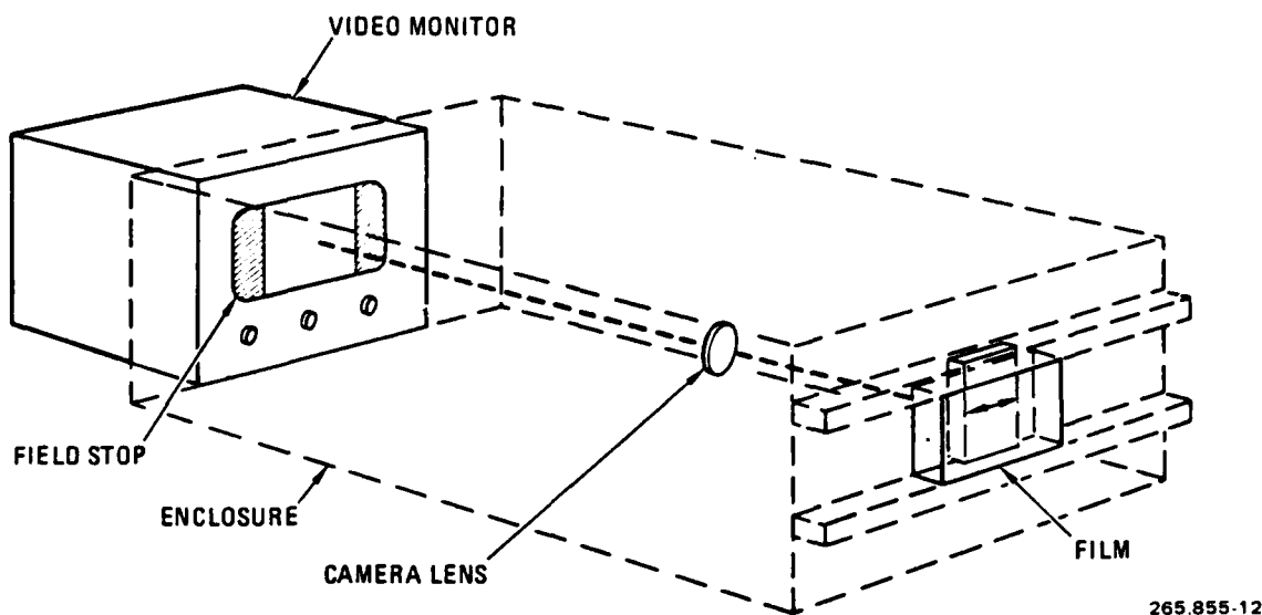
Figure 12. Slit Camera
