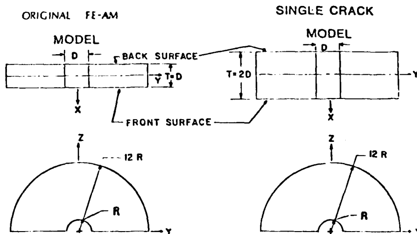
Fig. 2. Geometric models employed for uncracked solution in FEAM iterative algorithm. The half ring geometries shown were modeled by 112 3-dimensional finite elements.
