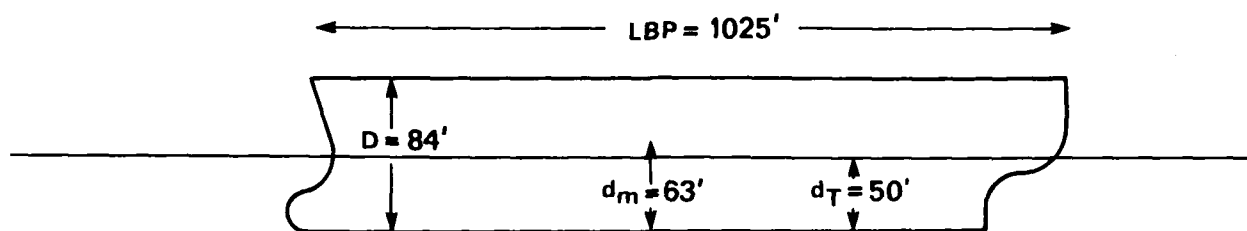
VESSEL ON AN EVEN KEEL - NO TRIM
