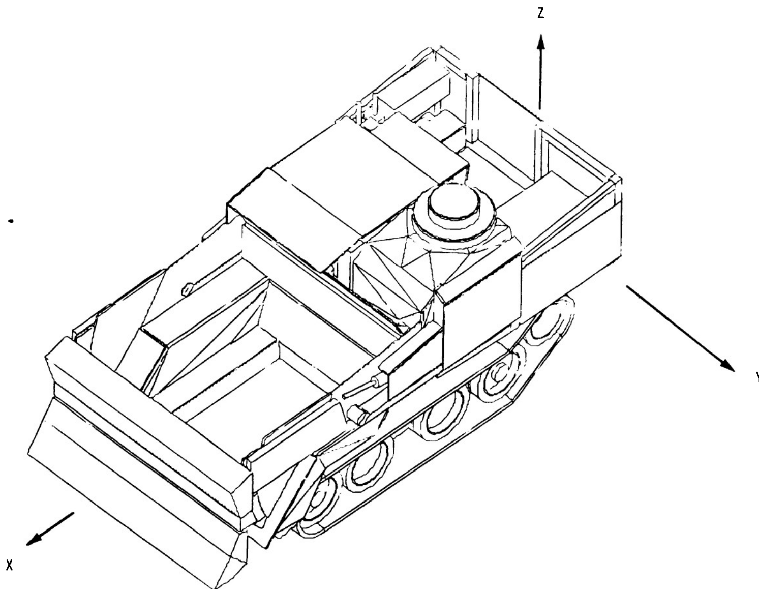
Figure 4. Coordinate System for COM-GEOM Description
