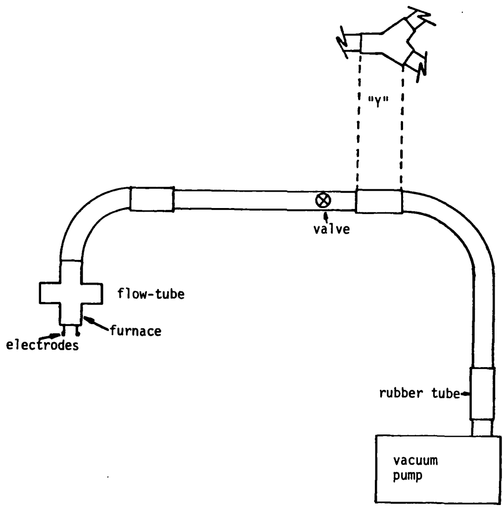
Figure 7. Vacuum System
