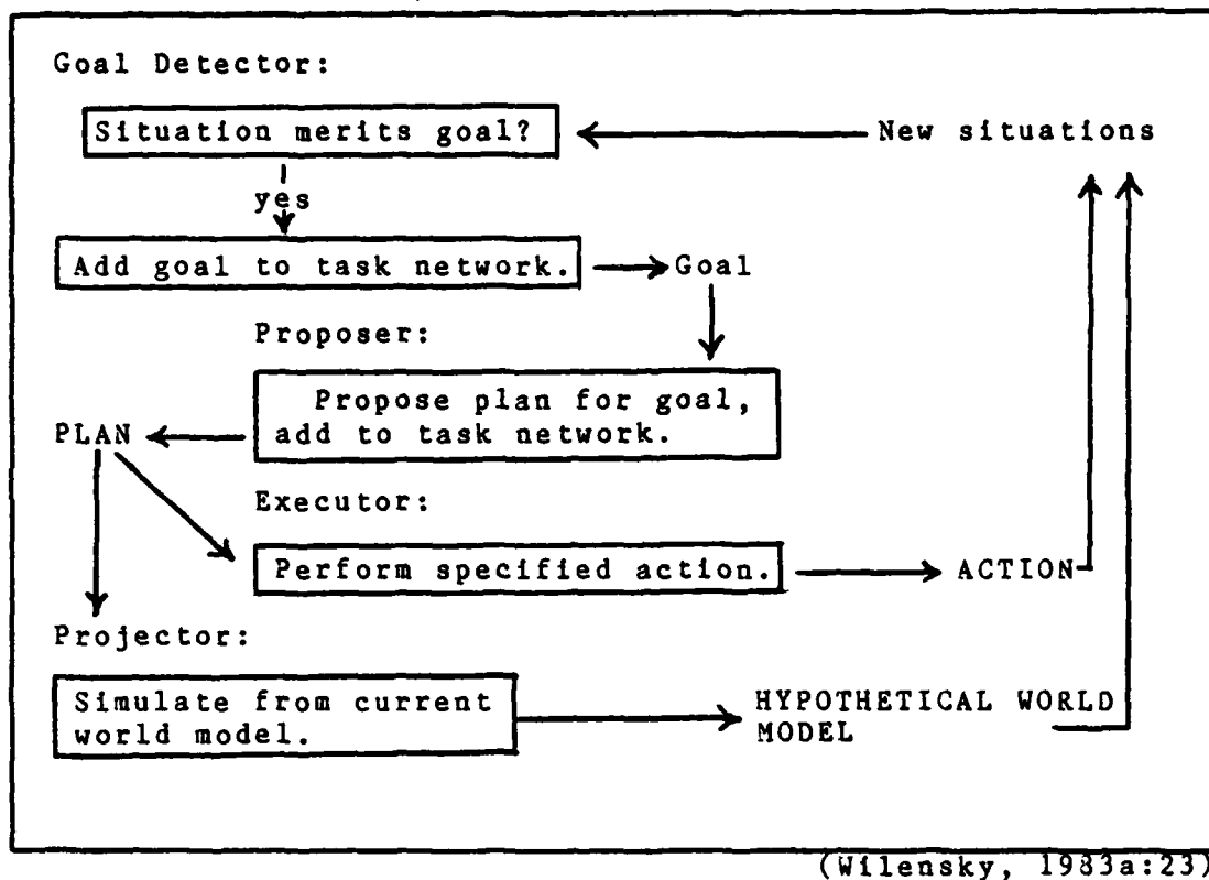
Figure 1. The Components of the Planner
