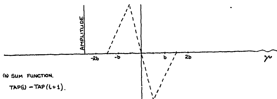
FIGURE; 4.10 CROSS CORRELATION FUNCTIONS, TIME-SHIFT MODULATION \left\{ TAP_L \left( \omega t = +1 \right), TAP_{L+1} \left( \omega t = -1 \right) \right\}
