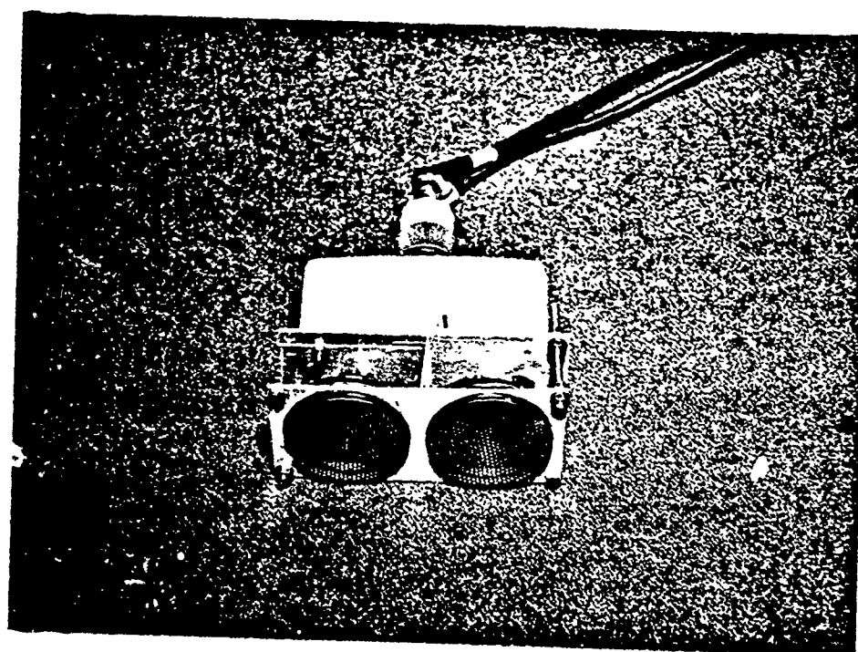
TRANSDUCER MODULE WITH POLAROID TRANSDUCERS (Type I and Type II systems)
