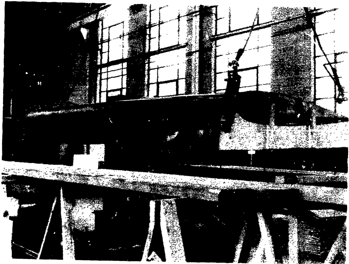
FIG. 5: MOULDED WOOD HURRICANE WING PANEL
