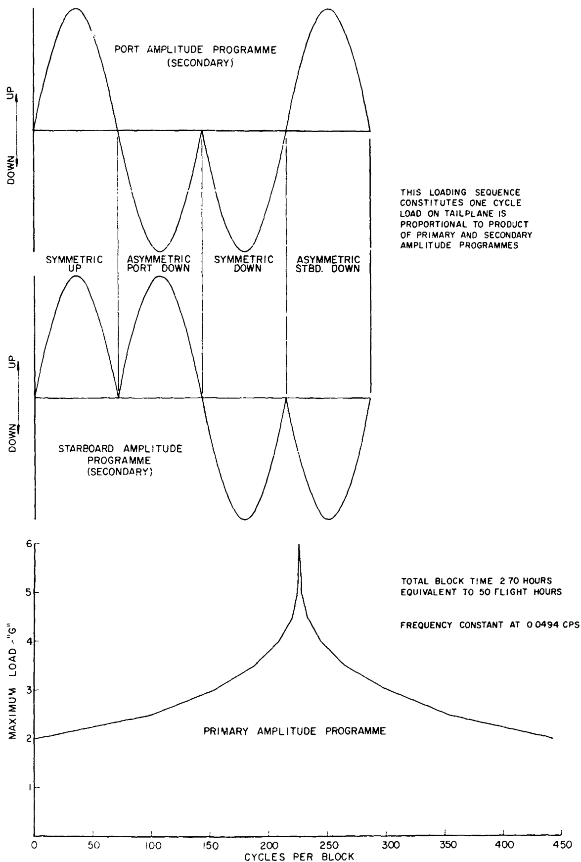
FIG. 33: TEST LOAD HISTORY FOR C-100 TAILPLANE
