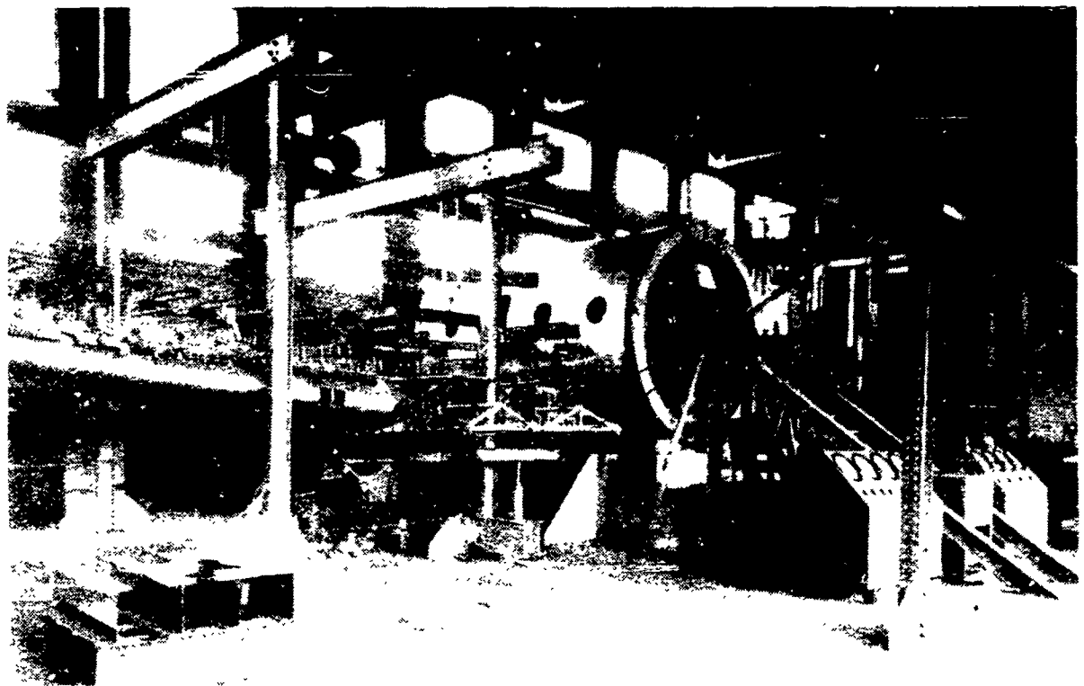
FIG. 20: TEST SET-UP FOR C-102 DERWENT MAINPLANE AND CENTRE FUSELAGE
