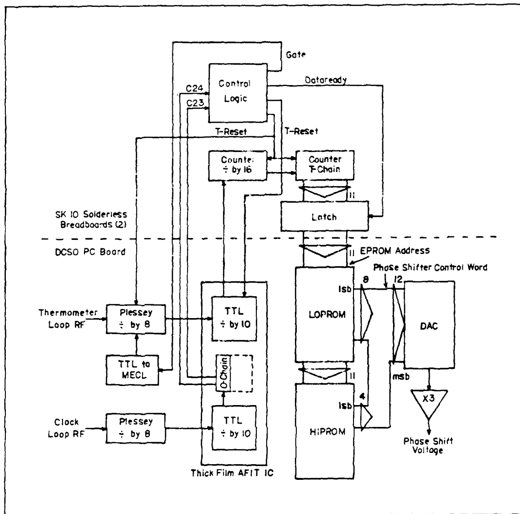
Figure VI-1. DCSO Control Circuitry Block Diagram
