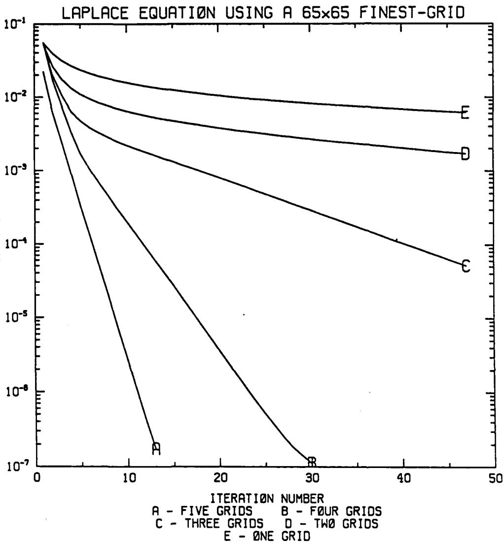
Figure 1a: Influence of grid levels on the convergence rate.
