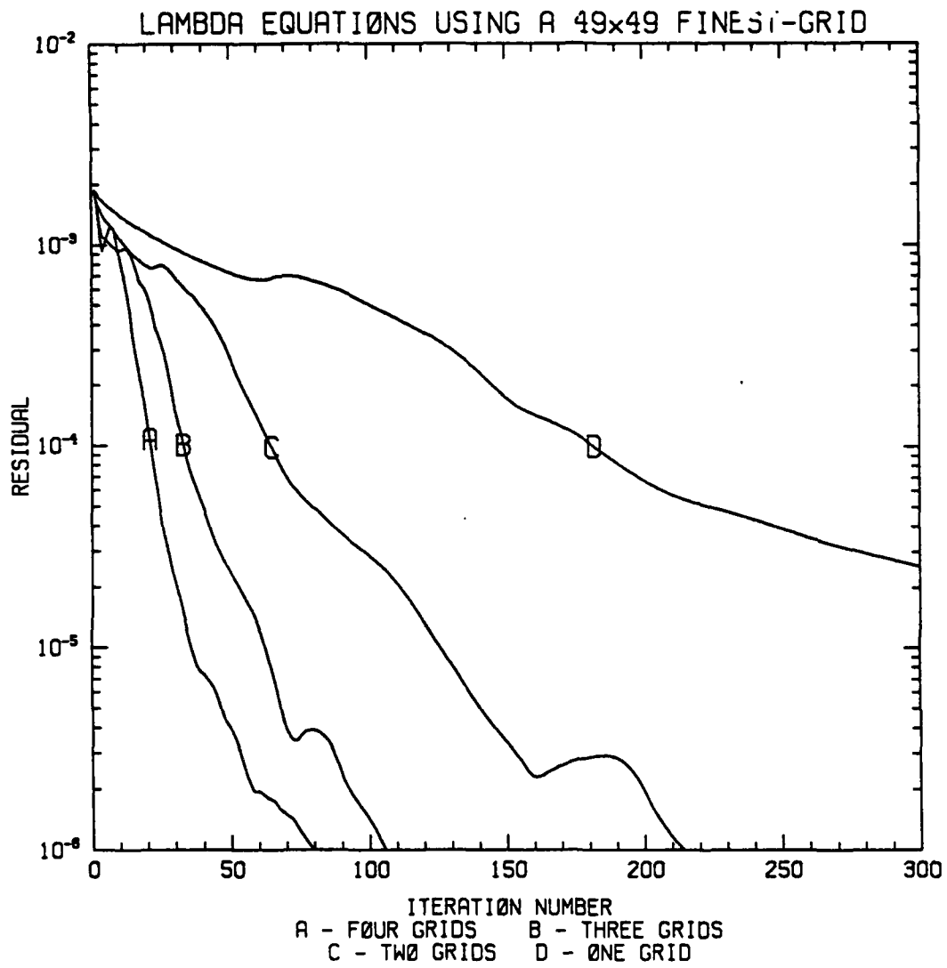
Figure 3b: Convergence history for the lambda equations
