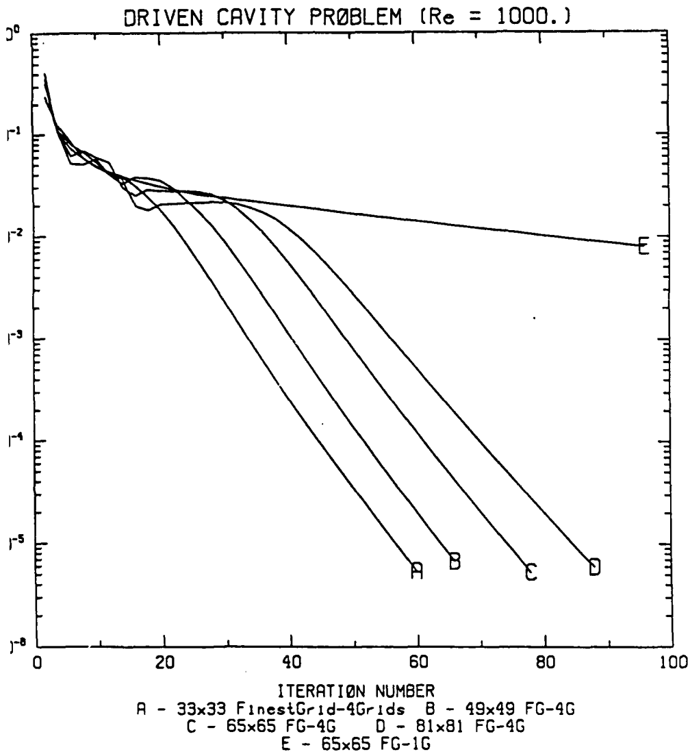
Figure 2: Convergence history for the Navier-Stokes equations
