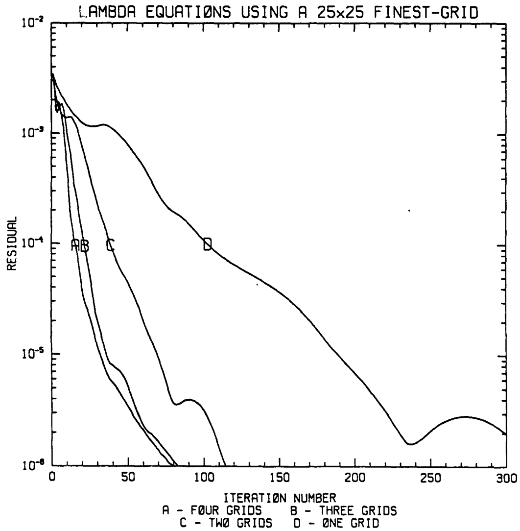
Figure 3a: Convergence history for the lambda equations
