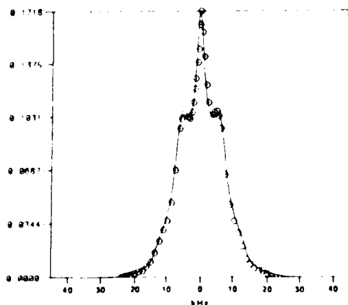
Figure 2. ^1\text{H} dipolar line shapes of \text{BPA-d}_6 in perdeutero-BPA. The points represent experimental data and the line the theoretical simulations in the high-temperature limit simulation.
