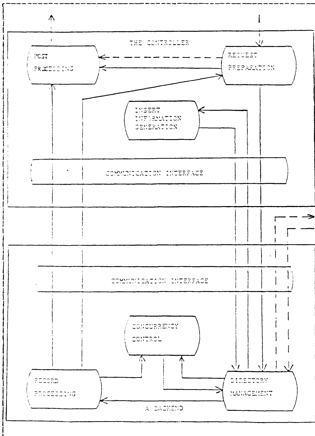
Figure 4.5 The MLBS Process Structure.
