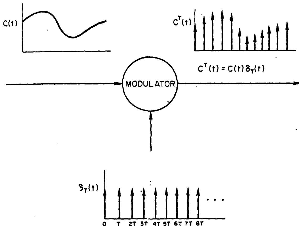
Figure 1. Amplitude Modulation of Impulse Train by Continuous Signal
